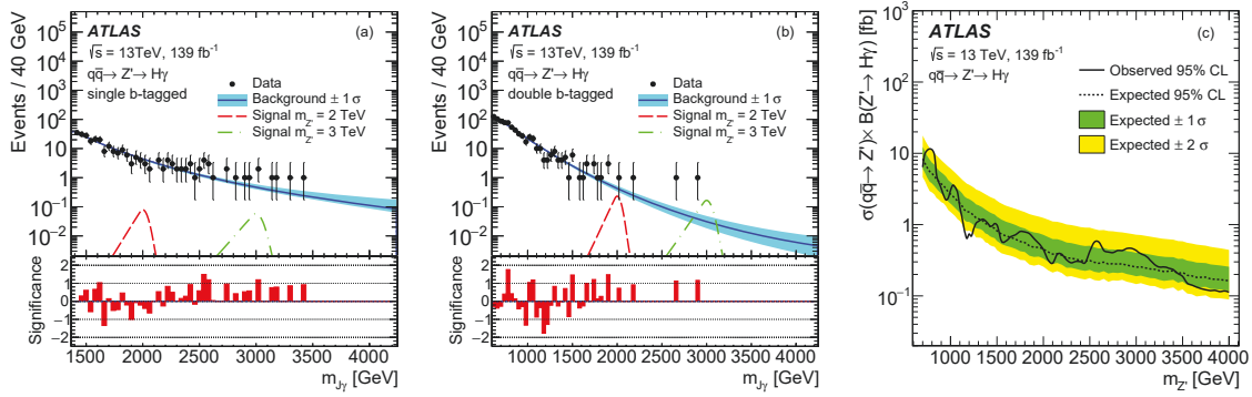
Figure 1: (a), (b) Distribution of the reconstructed m_{J\gamma} in the single- and double- b -tagged categories, with the background-only fits shown by the solid lines. The corresponding chi-square probabilities of the fits are 46% and 23%, after rebinning requiring at least five events in each bin. Hypothetical signal distributions for m_{Z'} = 2 TeV and m_{Z'} = 3 TeV with arbitrary normalizations are plotted for illustration purposes. The bottom panel gives the significance (deviation / statistical uncertainty) for each bin, calculated using the recommendation of Ref. [54]. The impact on the background fit from the statistical uncertainties of BPDF parameters is shown as a light band around the solid line. This effect is incorporated into the significance calculation. (c) Observed and expected 95% confidence-level limits on \sigma \times \mathcal{B} as a function of m_{Z'} .
