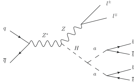
Figure 1: Representative tree-level Feynman diagram for the ZH production processes with the subsequent decays Z \rightarrow \ell\ell ( \ell = e, \mu ) and H \rightarrow aa \rightarrow (b\bar{b})(b\bar{b}) .
