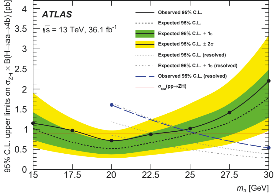
Figure 10: Summary of the 95% C.L. upper limits on \sigma_{ZH}\mathcal{B}(H \rightarrow aa \rightarrow (b\bar{b})(b\bar{b})) from this result and a previous search targeting the higher masses, labeled resolved [17]. The observed limits are shown together with the expected limits. In the case of the expected limits, one- and two-standard-deviation uncertainty bands are also displayed. The SM NNLO cross-section for pp \rightarrow ZH of 0.88 pb [66] is also shown.
