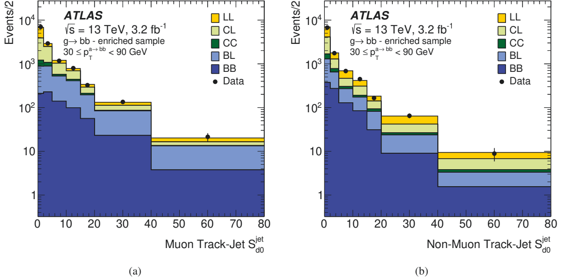
Figure 3: Averaged signed impact parameter significance S_{d0}^{\text{jet}} distributions of the track-jet (a) with a muon inside and (b) without a muon, after performing the fit of the flavor fractions to data. The total simulation yield is scaled to the same number of events observed in data. The fit is performed separately in p_T^{a \rightarrow b\bar{b}} ranges. The figure shows the 30 \text{ GeV} \leq p_T^{a \rightarrow b\bar{b}} < 90 \text{ GeV} range of a \rightarrow b\bar{b} candidates.
