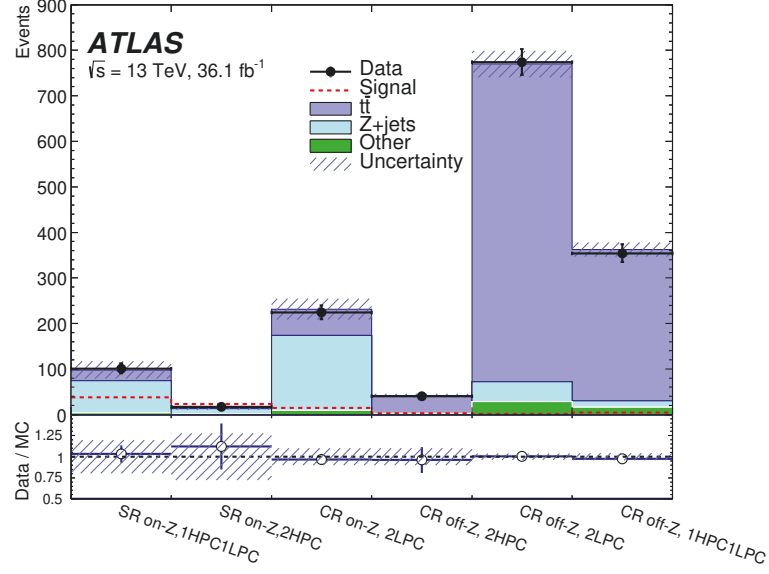
Figure 9: Expected yields for the different background components in each signal region (SR) and control region (CR) after the profile likelihood fit to data. The expected yield for signal with m_a = 20 GeV is calculated before the profile likelihood fit and normalized to the observed limit in the cross-section times the branching ratio for ZH , H \rightarrow aa \rightarrow (b\bar{b})(b\bar{b}) . The data observed in each region is included for comparison. The hashed area represents the total uncertainty in the background.
