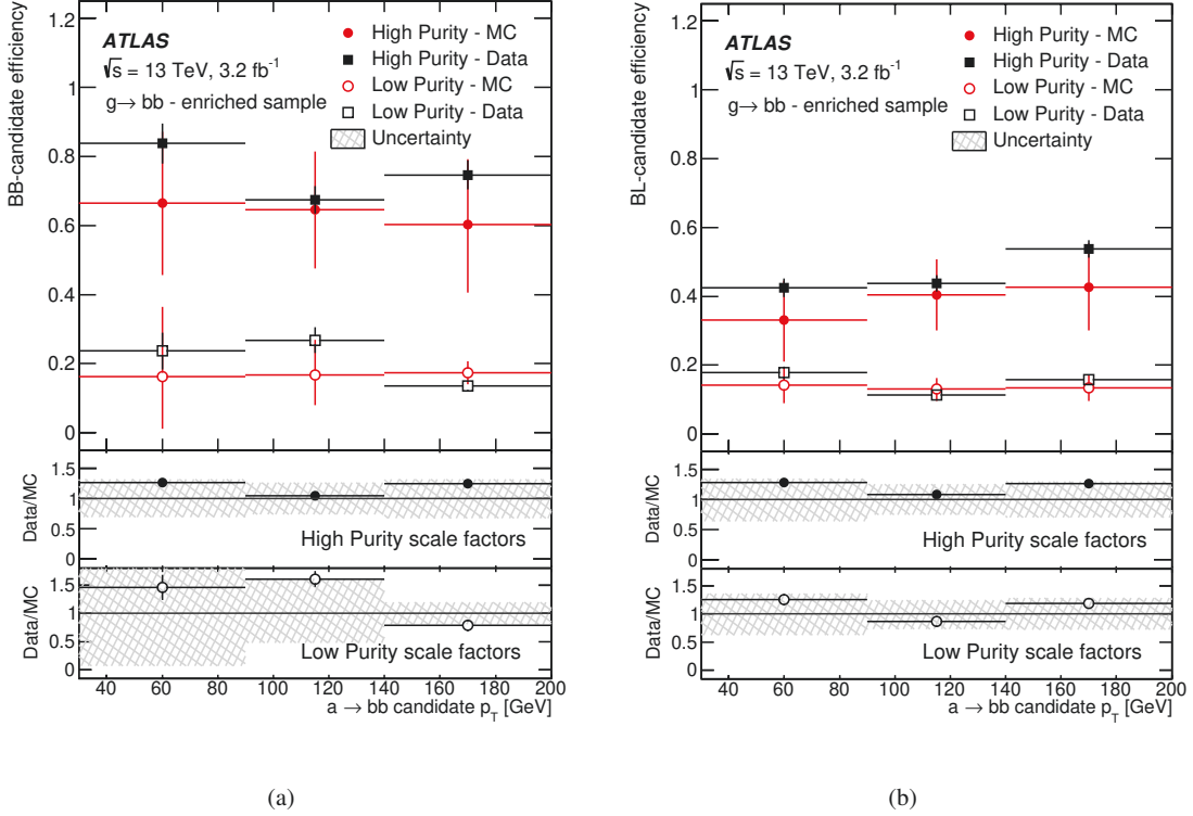
Figure 4: Efficiency of the a \rightarrow b\bar{b} identification criteria measured in data and simulated multijet events. The efficiency is measured in three transverse momentum ranges, separately for (a) BB and (b) BL candidates in both the HPC and LPC. The ratio of the measured values in data and simulation (bottom panels) are SFs used in the analysis when comparing simulation with data. The error bars in the top panels are statistical only, while the hashed bands on the ratios in the bottom panels include the full systematic uncertainties.
