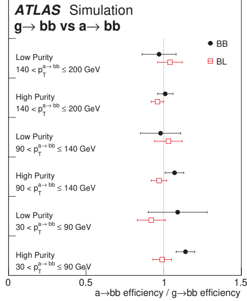
Figure 6: Efficiency measured using a simulated multijet pseudo-data where g \rightarrow b\bar{b} decays are replaced by a \rightarrow b\bar{b} decays with mass m_a = 20 GeV. The efficiency is measured separately for BB and BL samples in the same p_T ranges used in the data-to-simulation SF measurement. The values can be interpreted as the ratio between the SFs for a particle with mass m_a = 20 GeV and the ones for a massless gluon. Only the statistical uncertainties are indicated.
