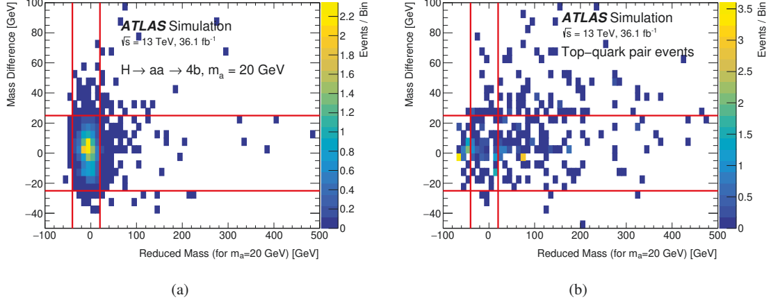
Figure 7: Distribution of (a) expected signal events and (b) top-quark pair background in a plane defined by the two mass requirements described in the text, m_{\text{red}} and \Delta m^{a \rightarrow b\bar{b}} . The mass requirements aim at selecting events where the two a \rightarrow b\bar{b} candidates have similar reconstructed masses and the mass of the pair of a \rightarrow b\bar{b} candidates is consistent with the Higgs boson mass. The signal events correspond to ZH, H \rightarrow aa \rightarrow (b\bar{b})(b\bar{b}) with m_a = 20 GeV and are normalized to the SM pp \rightarrow ZH cross-section.
