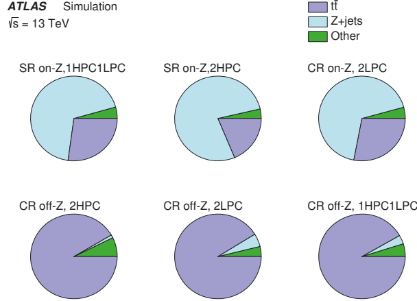
Figure 8: Expected composition of events in each signal region (SR) and control region (CR) defined for the search. CRs have a negligible expected yield for the signal. Definitions of the regions are based on the dilepton mass and the purity of the two a \rightarrow b\bar{b} candidates. Regions labeled “on-Z” require the dilepton mass to be in the range 85 \text{ GeV} < m_{\ell\ell} < 100 \text{ GeV} , while regions “off-Z” require the dilepton mass to be outside this window. For a \rightarrow b\bar{b} candidates, the HPC and LPC are defined using ranges of the identification BDT score, as described in Section 5.
