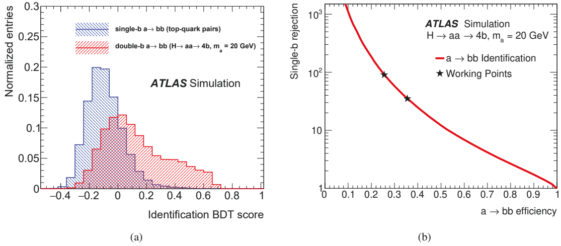
Figure 2: (a) Identification BDT score distributions for signal and background a \rightarrow b\bar{b} candidates and (b) signal efficiency as a function of the inverse of the t\bar{t} background efficiency (rejection). For the signal H \rightarrow aa \rightarrow (b\bar{b})(b\bar{b}) sample with m_a = 20 GeV, both b -quarks are required to lie within the reconstructed candidate, while for the background t\bar{t} sample the reconstructed candidate contains a single b -quark. In Figure (b), the left and right stars indicate the tight and the loose WPs, respectively, which are used to define, as described in the text, the HPC and LPC.
