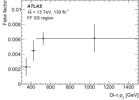
Figure 6: Fake factor as a function of the p_T of the di- \tau object, computed in the control region labelled as ‘FF SS’ in Table 2, with the requirements of Q = +1 for the di- \tau object and of zero b -tagged track-jets for the selected large- R jet. The error bars indicate the statistical uncertainties.
