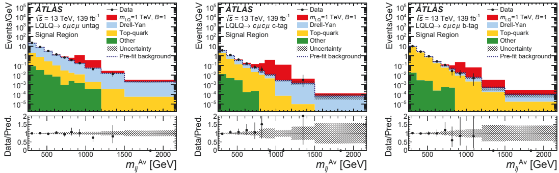
Figure 5: Post-fit distributions of m_{\ell j}^{Av} in the c\mu signal regions: untaged (left), c -tag (middle), and b -tag (right). The expected signals, shown for m_{LQ} = 1 TeV and \mathcal{B}(LQ \rightarrow c\mu) = 1 , are shown for illustrative purposes. The category ‘Top quark’ refers to t\bar{t} and single-top-quark processes. The category ‘Other’ refers to diboson and W +jet production. The hatched band represents the total uncertainty in the background predictions.
