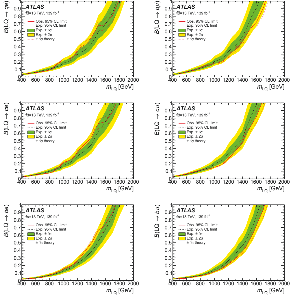
Figure 9: The observed (solid line) and expected (dashed line) limits on the leptoquark branching ratio \mathcal{B} into a quark and an electron or a muon at 95% CL, shown as a function of m_{LQ} for the different leptoquark channels. The green and yellow bands show the \pm 1\sigma and \pm 2\sigma ranges of the expected limit. The error band on the observed curve (dotted lines) represents the uncertainty in the theoretical cross-section from PDFs, renormalisation and factorisation scales, and the strong coupling constant \alpha_S .
