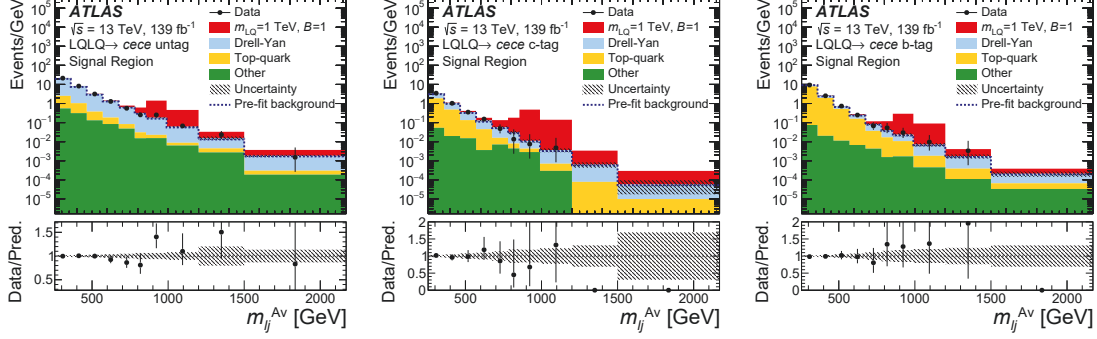
Figure 4: Post-fit distributions of m_{\ell j}^{Av} in the ce signal regions: untaged (left), c -tag (middle), and b -tag (right). The expected signals, shown for m_{LQ} = 1 TeV and \mathcal{B}(LQ \rightarrow ce) = 1 , are shown for illustrative purposes. The category ‘Top quark’ refers to t\bar{t} and single-top-quark processes. The category ‘Other’ refers to diboson and W +jet production. The hatched band represents the total uncertainty in the background predictions.
