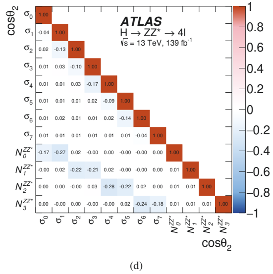
Figure 22: Differential fiducial cross sections for (a) production angle, \cos\theta_1 , of the anti-lepton from the leading Z boson and (c) the production angle, \cos\theta_2 , of the anti-lepton from the subleading Z boson. The corresponding correlation matrices between the measured cross sections and the ZZ^* background normalisation factors are also shown ((b) and (d)).
