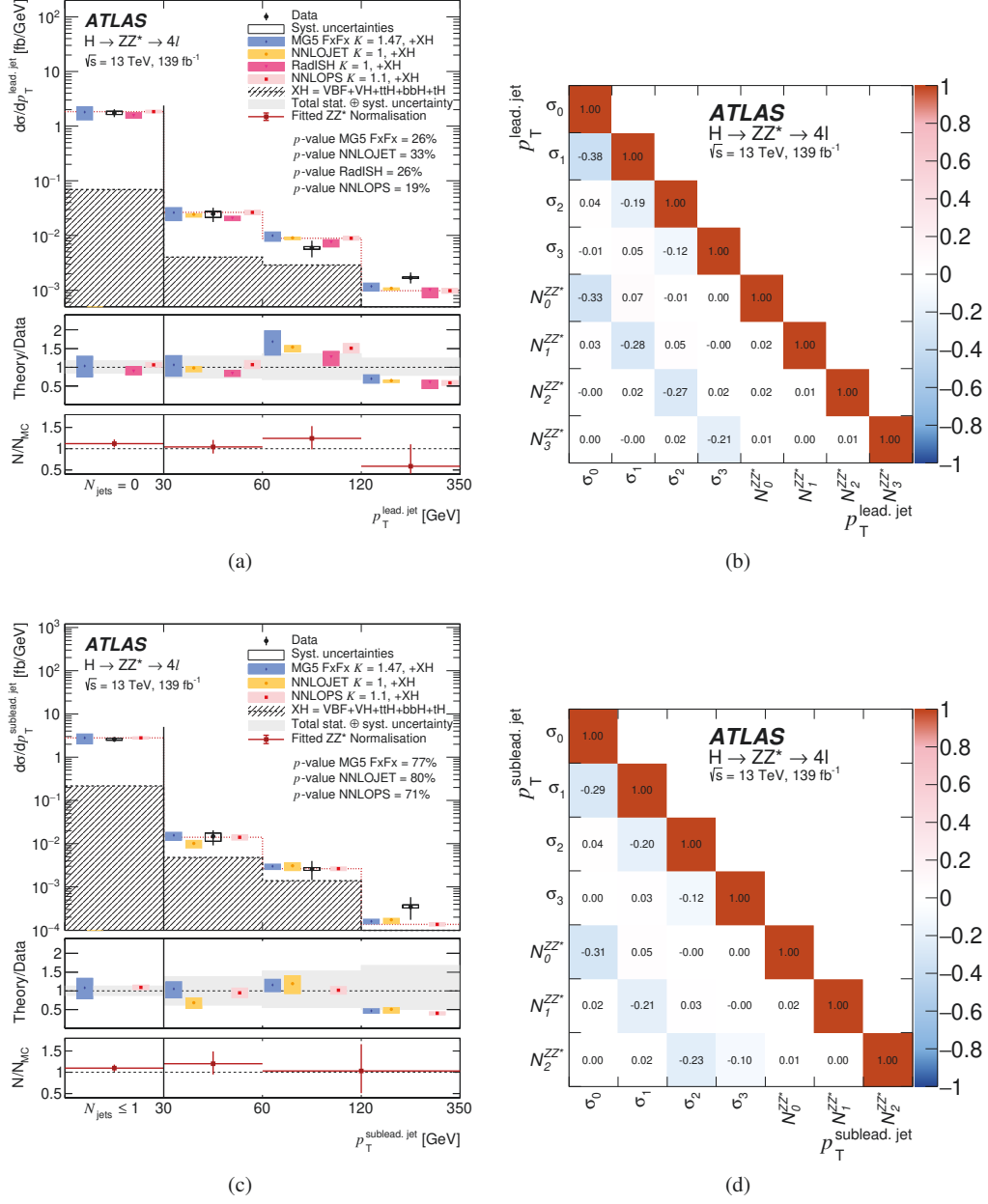
Figure 26: Differential fiducial cross sections for (a) the transverse momentum of the leading jet, p_T^{\text{lead, jet}} , in events with at least one jet, and (c) the transverse momentum of the subleading jet, p_T^{\text{sublead, jet}} , in events with at least two jets. Leading and subleading jets refer to the jets with the highest and second-highest transverse momenta. The first bin contains events which do not pass the jet requirements. The corresponding correlation matrices between the measured cross sections and the ZZ^* background normalisation factors are also shown ((b) and (d)).
