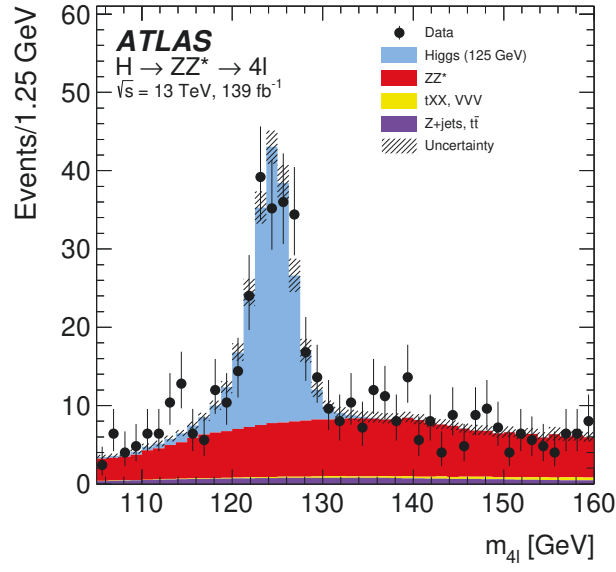
Figure 2: The observed and expected (pre-fit) inclusive four-lepton invariant mass distributions for the selected Higgs boson candidates, shown for an integrated luminosity of 139 \text{ fb}^{-1} and at \sqrt{s} = 13 \text{ TeV} . The uncertainty in the prediction is shown by the hatched band, which includes the theoretical uncertainties of the SM cross section for the signal and the ZZ^* background.
