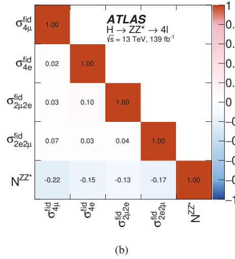
Figure 18: (a) The fiducial cross sections (left two panels) and total cross section (right panel) of Higgs boson production measured in the 4\ell final state. The fiducial cross sections are shown separately for each decay final state, and for same- and different-flavour decays. The inclusive fiducial cross section is measured as the sum of all final states, as well as by combining the per-final-state measurements assuming SM ZZ^* \rightarrow 4\ell relative branching ratios. The total SM prediction is accurate to N^3\text{LO} in QCD for the ggF process. The cross sections for all other Higgs boson production modes XH are added. For the fiducial cross-section predictions, the SM cross sections are multiplied by the acceptances determined using the NNLOPS sample for ggF and the samples discussed in Section 3 for the other production modes. For the total cross section, the predictions by the generators NNLOPS, HRes, and MADGRAPH5_AMC@NLO-FxFx are also shown. The error bars on the data points show the total uncertainties, while the systematic uncertainties are indicated by the boxes. The shaded bands around the theoretical predictions indicate the PDF and scale uncertainties, calculated as described in Section 8.2. (b) The correlation between the fiducial cross sections for the four individual decay final states and the ZZ^* normalisation factor.
