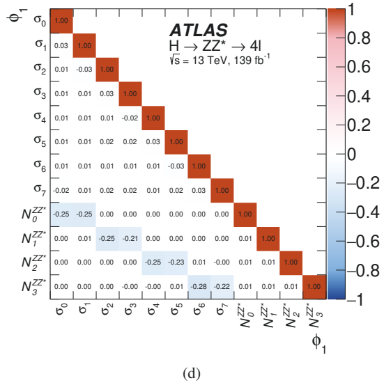
Figure 23: Differential fiducial cross sections for (a) the azimuthal angle, \phi , between the decay planes of the two reconstructed Z bosons and (c) the azimuthal angle, \phi_1 , between the decay plane of the leading Z boson and the plane formed by its four-momentum and the z -axis. The corresponding correlation matrices between the measured cross sections and the ZZ^* background normalisation factors are also shown ((b) and (d)).
