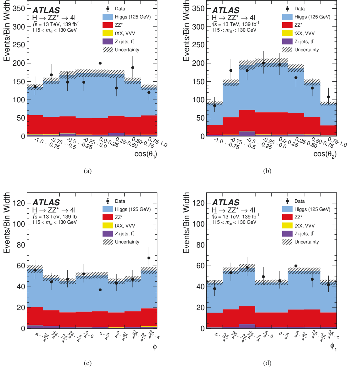
Figure 6: The observed and expected (pre-fit) distributions of (a) \cos \theta_1 , (b) \cos \theta_2 , (c) \phi , and (d) \phi_1 in the mass region 115 < m_{4\ell} < 130 GeV, for an integrated luminosity of 139 \text{ fb}^{-1} collected at \sqrt{s} = 13 TeV. A SM Higgs boson signal with a mass m_H = 125 GeV is assumed. The uncertainty in the prediction is shown by the hatched band, which includes the theoretical uncertainties of the SM cross section for the signal and the ZZ^* background.
