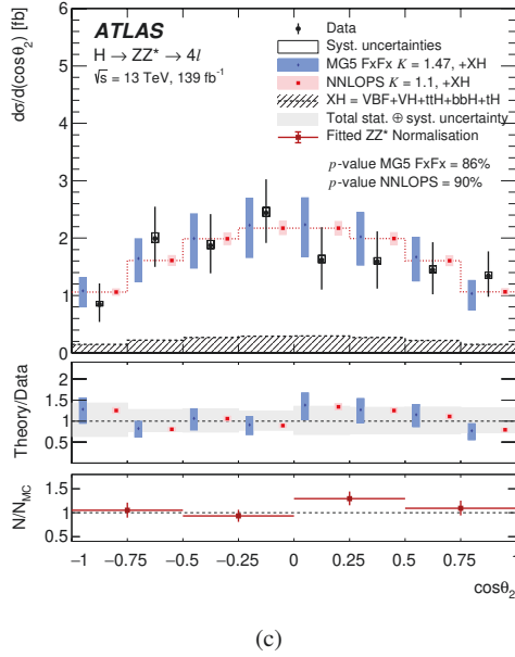
Figure 22: Differential fiducial cross sections for (a) production angle, \cos\theta_1 , of the anti-lepton from the leading Z boson and (c) the production angle, \cos\theta_2 , of the anti-lepton from the subleading Z boson. The corresponding correlation matrices between the measured cross sections and the ZZ^* background normalisation factors are also shown ((b) and (d)).
