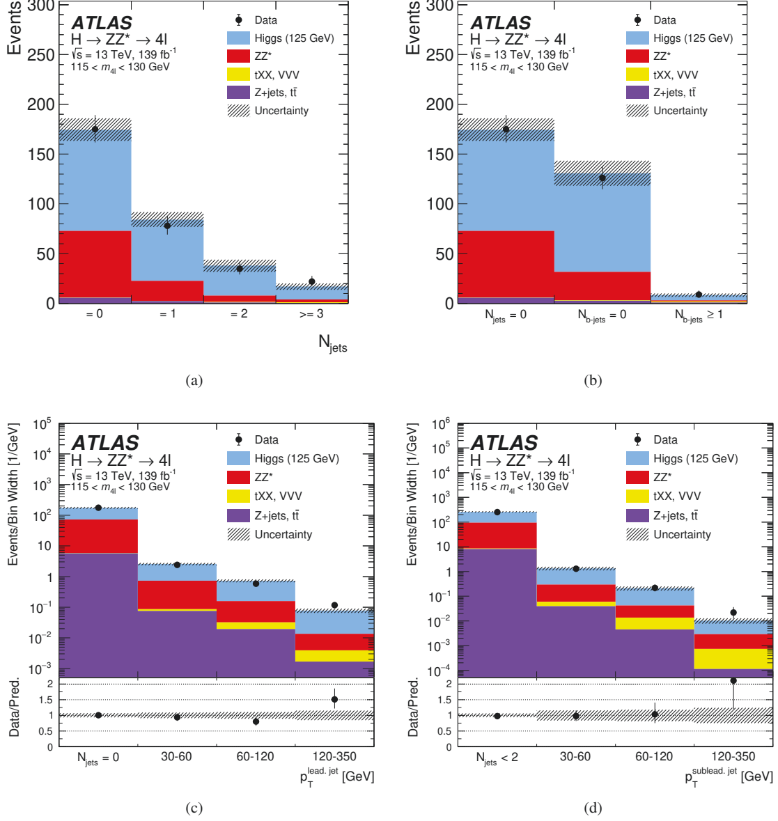
Figure 7: The observed and expected (pre-fit) distributions of (a) N_{\text{jets}} , (b) N_{b\text{-jets}} , (c) p_T^{\text{lead. jet}} , and (d) p_T^{\text{sublead. jet}} in the mass region 115 < m_{4l} < 130 GeV, for an integrated luminosity of 139 \text{ fb}^{-1} collected at \sqrt{s} = 13 TeV. A SM Higgs boson signal with a mass m_H = 125 GeV is assumed. In distribution (c), the first bin contains events with zero jets, while in distribution (d), the first bin contains events with fewer than two jets. In both (c) and (d), all bins except the first are divided by the bin width. The uncertainty in the prediction is shown by the hatched band, which includes the theoretical uncertainties of the SM cross section for the signal and the ZZ^* background.
