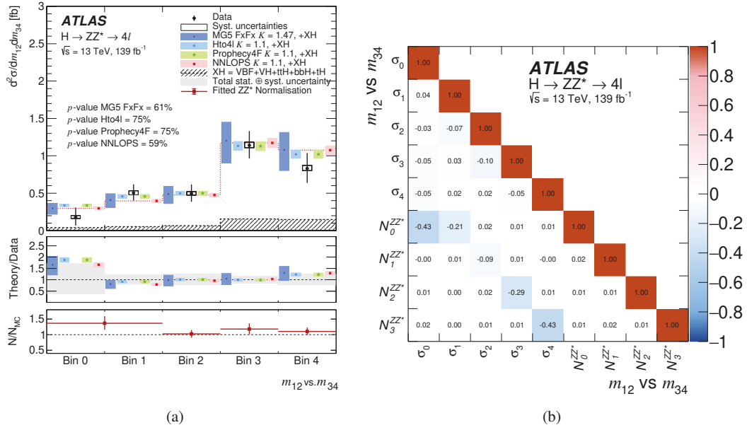
Figure 31: (a) Differential fiducial cross section for the leading vs. subleading Z boson mass, m_{12} vs. m_{34} , and (b) the corresponding correlation matrix between the measured cross sections and the ZZ^* background normalisation factors. The bin boundaries are defined in Figure 12.
