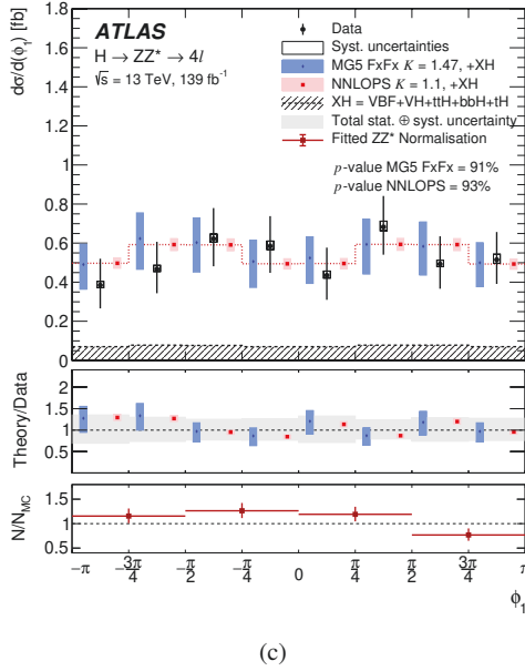
Figure 23: Differential fiducial cross sections for (a) the azimuthal angle, \phi , between the decay planes of the two reconstructed Z bosons and (c) the azimuthal angle, \phi_1 , between the decay plane of the leading Z boson and the plane formed by its four-momentum and the z -axis. The corresponding correlation matrices between the measured cross sections and the ZZ^* background normalisation factors are also shown ((b) and (d)).
