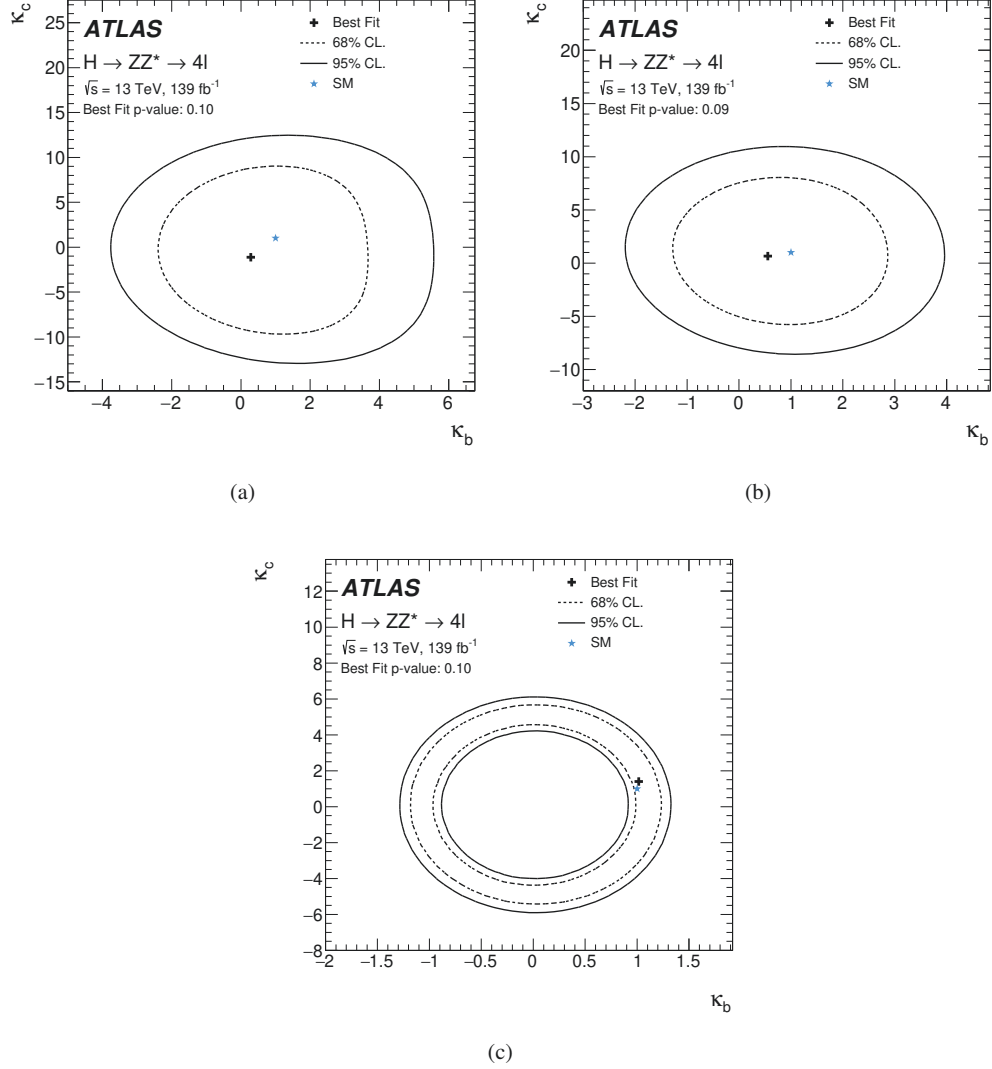
Figure 41: Observed limits at 95% CL on Yukawa couplings \kappa_c and \kappa_b for the three scenarios considered: (a) only the p_T^{4\ell} shape is used to constrain \kappa_c and \kappa_b ; (b) the predicted p_T^{4\ell} differential cross section is used; (c) both the prediction of the p_T^{4\ell} differential cross section and the modification to the branching ratio due to the \kappa_c and \kappa_b values are used. The p -values shown represent the probability of compatibility between the data and the p_T^{4\ell} prediction corresponding to the best-fit values of \kappa_c and \kappa_b . The SM predictions (*) and the observed best-fit values (+) are indicated on the plots.
