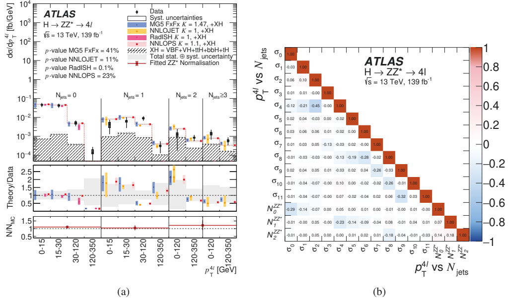
Figure 34: (a) Double differential fiducial cross sections of the p_T^{4\ell} distribution in N_{jets} bins. The corresponding correlation matrix between the measured cross sections and the ZZ^* background normalisation factors is shown in (b). The p -values shown are calculated for all bins across both p_T^{4\ell} and N_{jets} simultaneously.
