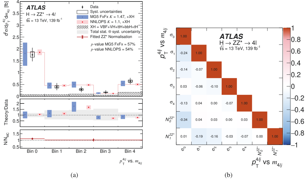
Figure 36: (a) Double differential fiducial cross section for the transverse momentum of the four-lepton plus jet system vs. the invariant mass of the four-lepton plus jet system, p_T^{4\ell j} vs. m_{4\ell j} and (b) the corresponding correlation matrix between the measured cross sections and the ZZ^* background normalisation factors. The bin boundaries are defined in Figure 13.
