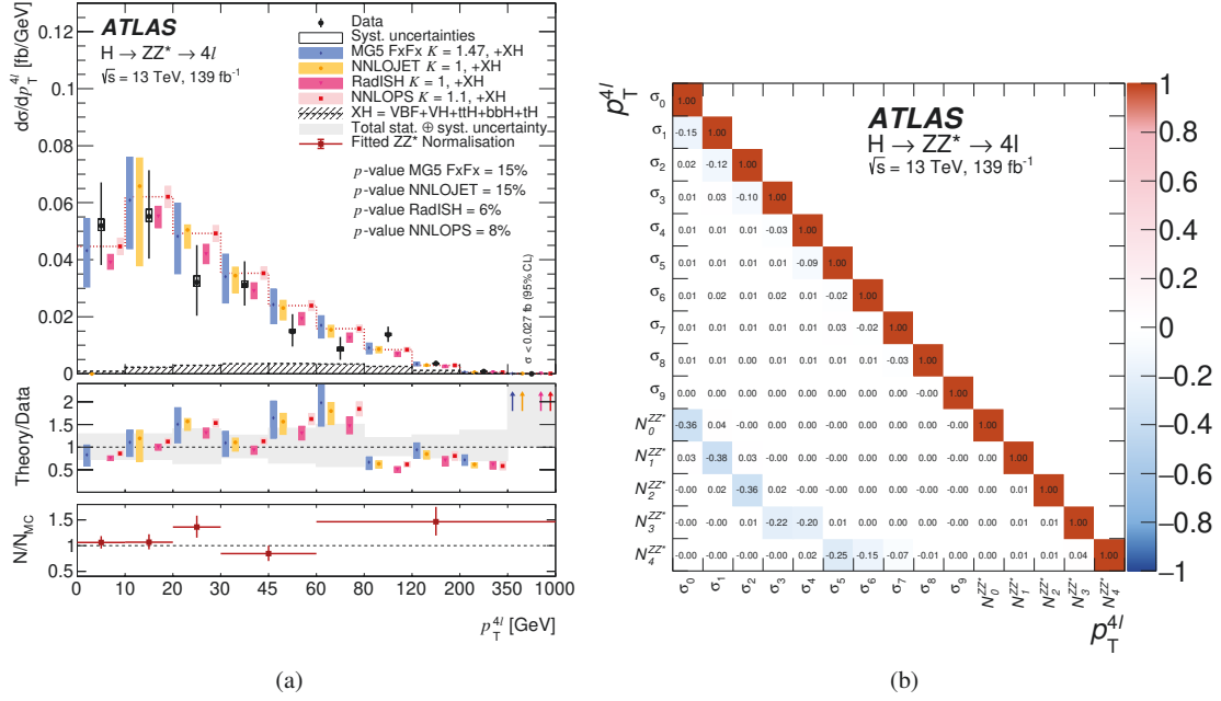
Figure 19: (a) Differential fiducial cross section for the transverse momentum p_T^{4\ell} of the Higgs boson, along with (b) the corresponding correlation matrix between the measured cross sections and the ZZ^* background normalisation factors. The measured cross sections are compared with ggF predictions by MADGRAPH5_AMC@NLO-FxFx, NNLOJET, RADISH, and NNLOPS, where MADGRAPH5_AMC@NLO-FxFx and NNLOPS are normalised to the N 3 LO total cross section with the listed K -factors while the normalisations for NNLOJET and RADISH are to their respective predicted cross sections. MC-based predictions for all other Higgs boson production modes XH are normalised to the SM predictions. The error bars on the data points show the total uncertainties, while the systematic uncertainties are indicated by the boxes. The shaded bands on the expected cross sections indicate the PDF and scale systematic uncertainties, calculated as described in Section 8.2. This includes the uncertainties related to the XH production modes. The p -values indicating the probability of compatibility of the measurement and the SM prediction are shown as well. They do not include the systematic uncertainty in the theoretical predictions. The central panel of (a) shows the ratio of different predictions to the data, and the grey area represents the total uncertainty of the measurement. The bottom panel of (a) shows the ratios of the fitted values of the ZZ^* normalisation factors to the predictions from MC simulation discussed in Section 3. As indicated by the horizontal error bars, the ZZ^* normalisation is estimated in each of the first three p_T^{4\ell} bins separately, while the next two bins share a common estimation factor, as do the last five bins.
