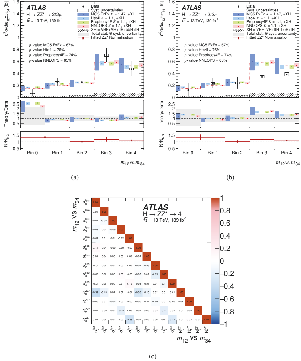
Figure 32: Differential fiducial cross sections for the leading vs. subleading Z boson mass, m_{12} vs. m_{34} , in (a) \ell\ell\mu\mu and (b) \ell\ell ee final states, along with (c) their corresponding correlation matrix between the measured cross sections and the ZZ^* background normalisation factors. The bin boundaries are defined in Figure 12.
