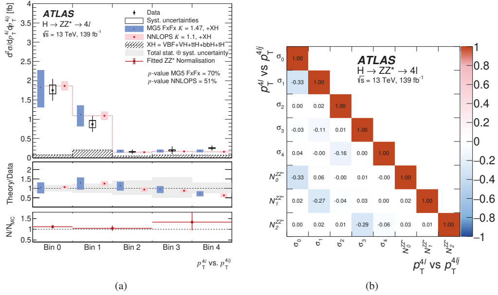
Figure 35: (a) Differential fiducial cross section for the transverse momentum of the four-lepton system vs. the transverse momentum of the four-lepton plus jet system, p_T^{4\ell} vs. p_T^{4\ell j} and (b) the corresponding correlation matrix between the measured cross sections and the ZZ^* background normalisation factors. The bin boundaries are defined in Figure 14.
