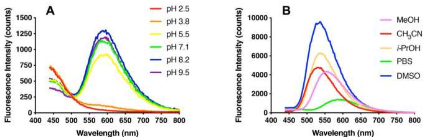
Figure 3. Solvent effects on Dad fluorescence. A. Emission spectra of 5 \mu M Dad in CBTP buffer at various pHs ( \lambda_{\text{Ex}} 425 nm). B. Emission spectra of 5 \mu M Dad in various solvents ( \lambda_{\text{Ex}} 425 nm).
