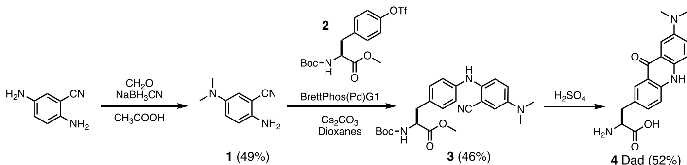
Scheme 1. Synthesis of Dad.
