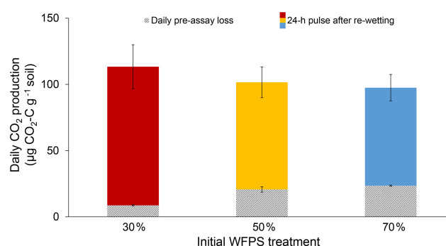
Figure 3. Daily CO 2 production rates for each initial WFPS treatment. Lined bars represent the average daily rate of pre-assay CO 2 loss during a 3 d dry-down period and solid bars represent the 24 h CO 2 pulses after re-wetting the air-dried soil. Together both bars represent the 24 h CO 2 pulse corrected for pre-assay losses of CO 2 during dry-down. Error bars represent standard deviation, which was calculated based on bootstrap error propagation for the daily pre-assay losses.
