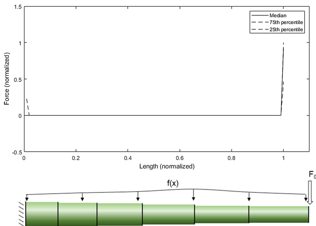
Fig. 12 The drag force profile for all 945 specimens ( f(x) and F_0 ) (top); a loading diagram of f(x) and F_0 (bottom). The 75th and 25th percentile values are generally line-on-line with the median values along the length of the specimen. Plant height (x-axis) is normalized to the height of the plant specimen. Force (y-axis) is normalized to the maximum calculated force
