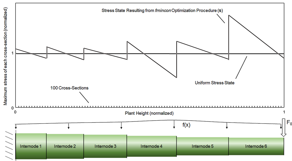
Fig. 3 A typical specimen output, showing the stress state resulting from the fmincon optimization procedure, which attempts to create the most uniform possible stress state along the length of the specimen by altering values for F_0 and f(x) (top); the analytical maize stalk model partitioned into 100 cross-sections along its length (bottom). Plant height (x-axis) is normalized to the height of the plant specimen. Maximum stress of each cross-section (y-axis) normalized to a target stress of 1.00
