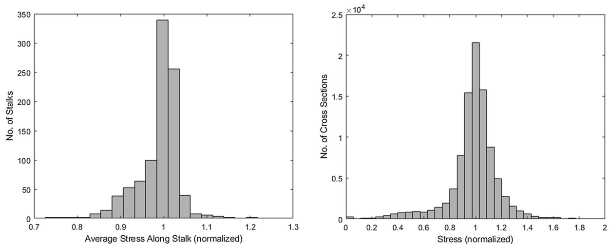
Fig. 7 A histogram of the average stress along the length of each of the 945 specimens after optimization, n = 945 (left); a histogram of the average stress at all 100 cross-sections along the length of each of the 945 specimens after optimization, n = 94,500 (right). All stress are normalized to a target stress of 1.00. Thus, stress states that deviate from 1.00 represent a suboptimal structural allocation of biomass
