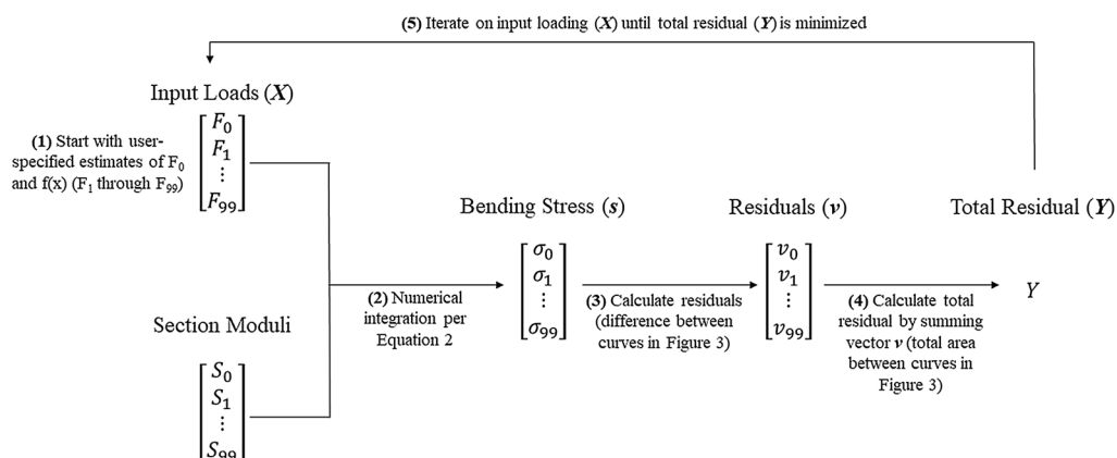
Fig. 4 A flowchart of the optimization algorithm procedure
