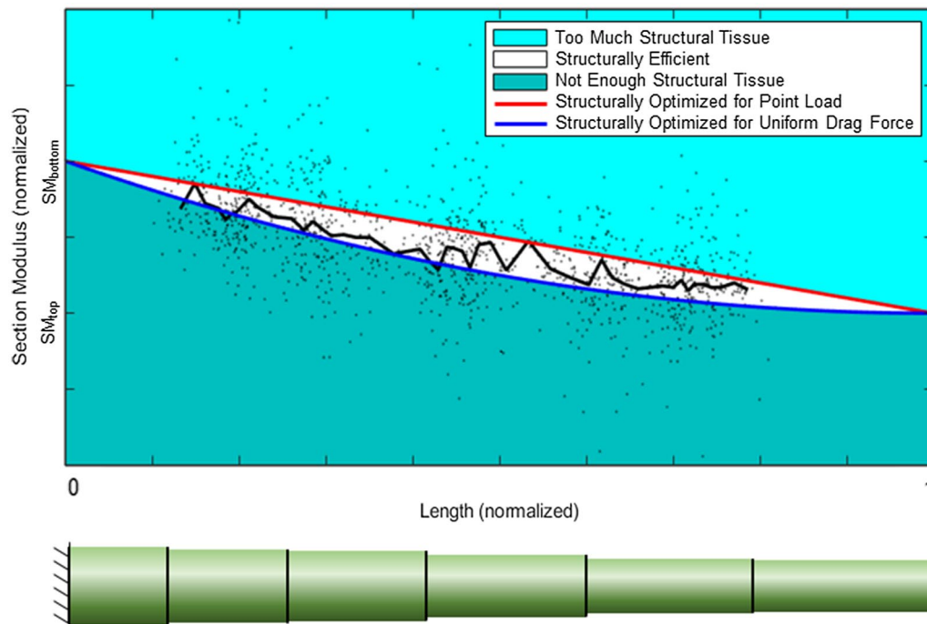
Fig. 6 The measured section moduli of the specimens as compared to the region of structural efficiency. Section modulus (y-axis) is normalized by the difference between the section modulus at the top internode ( SM_{top} ) and the bottom internode ( SM_{bottom} )
