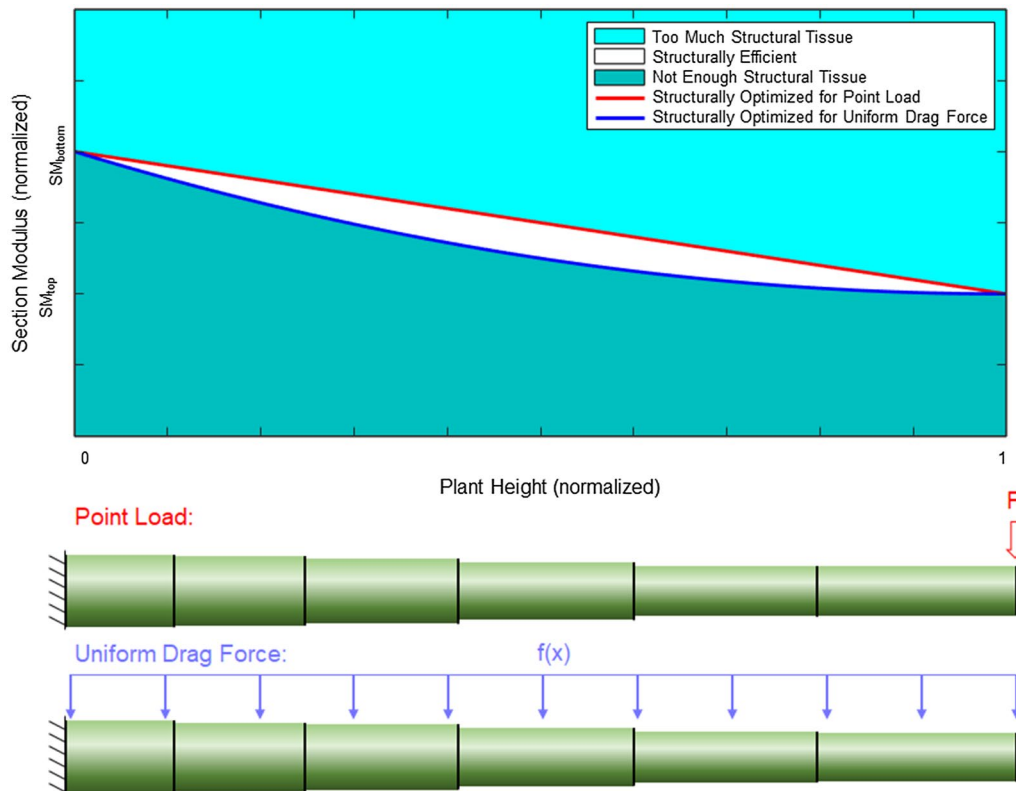
Fig. 1 Structural efficiency along the length of the specimen as a function of probable wind loadings (top); loading diagrams for a point load and uniform drag force (bottom). Plant height (x-axis) is normalized to the height of the plant specimen. Section modulus (y-axis) is normalized by the difference between the section modulus at the top internode ( SM_{top} ) and the bottom internode ( SM_{bottom} )
