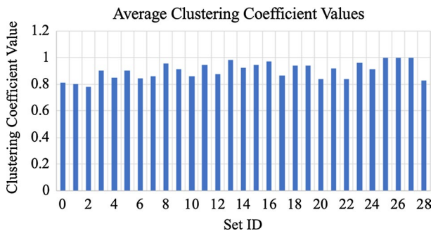
Fig. 12 Focal structure sets' average clustering coefficient values
