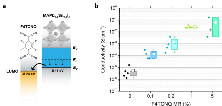
Fig. 1 (a) Band diagram of the \text{MAPb}_{0.5}\text{Sn}_{0.5}\text{I}_3 perovskite host and F4TCNQ molecular p-dopant, illustrating charge transfer from the top of the perovskite valence band ( E_v ) to the LUMO of the dopant. Upon efficient charge transfer, the Fermi level E_f is shifted toward the valence band. The perovskite E_v is measured by UPS in this study. (b) \text{MAPb}_{0.5}\text{Sn}_{0.5}\text{I}_3 conductivity for different F4TCNQ molar ratio (MR) concentrations. Several samples have been measured for each dopant concentration and the box charts indicate the maximum and minimum values (whiskers), the upper quartile and lower quartile (box) and the mean value (empty square).
