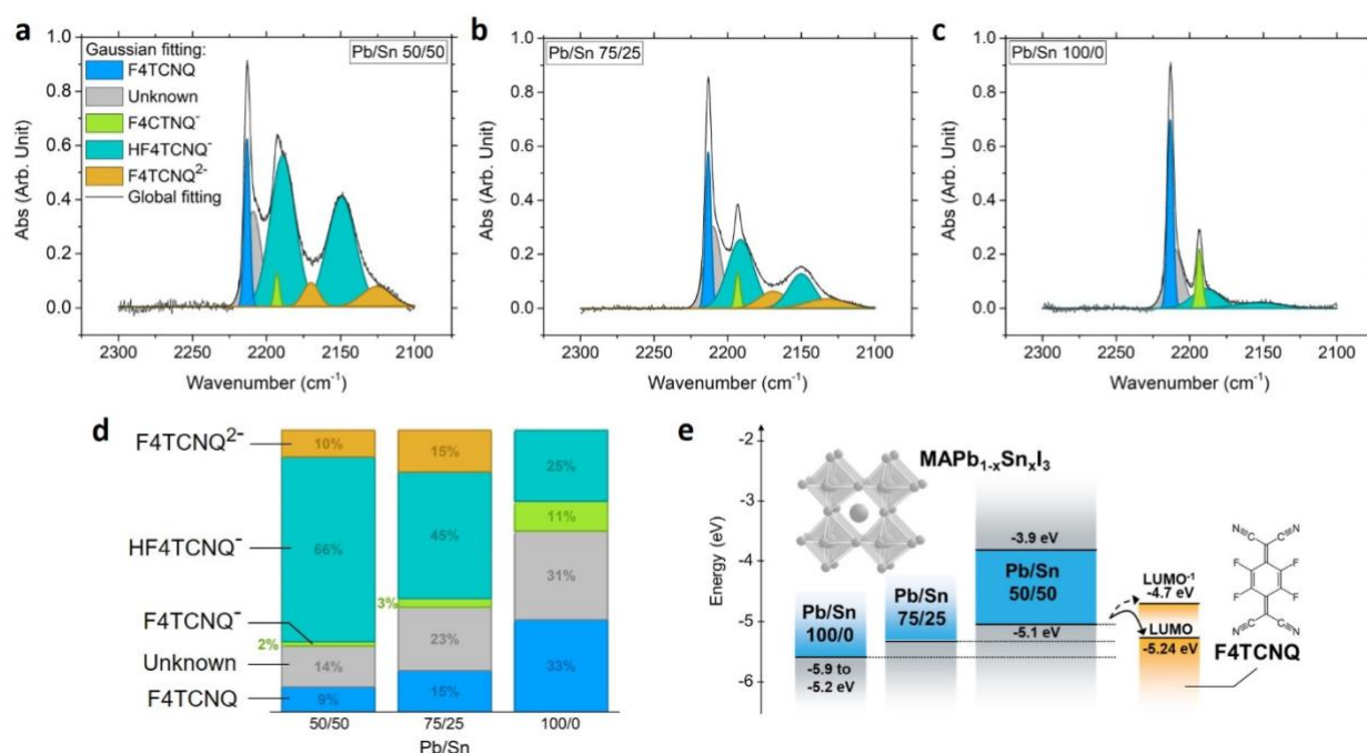
Fig. 5 FTIR absorption spectra of the F4TCNQ cyano groups for 5% MR doped MAPb 1-x Sn x I 3 with Pb/Sn ratio of 50/50 ( x =0.5) (a), 75/25 ( x =0.25) (b) and 100/0 ( x =0) (c). (d) Area under the curve associated with F4TCNQ, F4TCNQ - , HF4TCNQ - , F4TCNQ 2- and an unknown component, from the Gaussian fitting of the FTIR spectra. See Fig. S15 for the extraction of peak position and area. (e) Band diagram schematic showing the LUMO of neutral and singly ionized F4TCNQ (LUMO -1 ), 19,32 the VBM and CBM of MAPb 0.5 Sn 0.5 I 3 from UPS and absorption measurements measured in this study, and a schematic view of the VBM evolution for MAPb 0.75 Sn 0.25 I 3 and MAPbI 3 . 25,26,38,39,60
