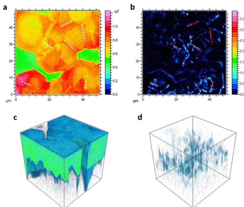
Fig. 3 TOF-SIMS 2D images of 1% doped MAPb 0.5 Sn 0.5 I 3 exhibiting the total signal (a) and the F signal (b). Each image is 50x50 μm and the color scale for each image shows the intensity in counts/pixel. The yellow-green area in panel (a) corresponds to uncoated glass substrate. White and red dotted lines are drawn as guide to the eye to show examples of grain boundaries visible in the total (a) and F (b) signals. TOF-SIMS 3D tomography rendering of the same dataset showing the signal coming from MA (MA: methylammonium), indicating the presence of the perovskite (c) and the F signal (d). Each 3D reconstruction is 50 × 50 × film thickness μm 3 .
