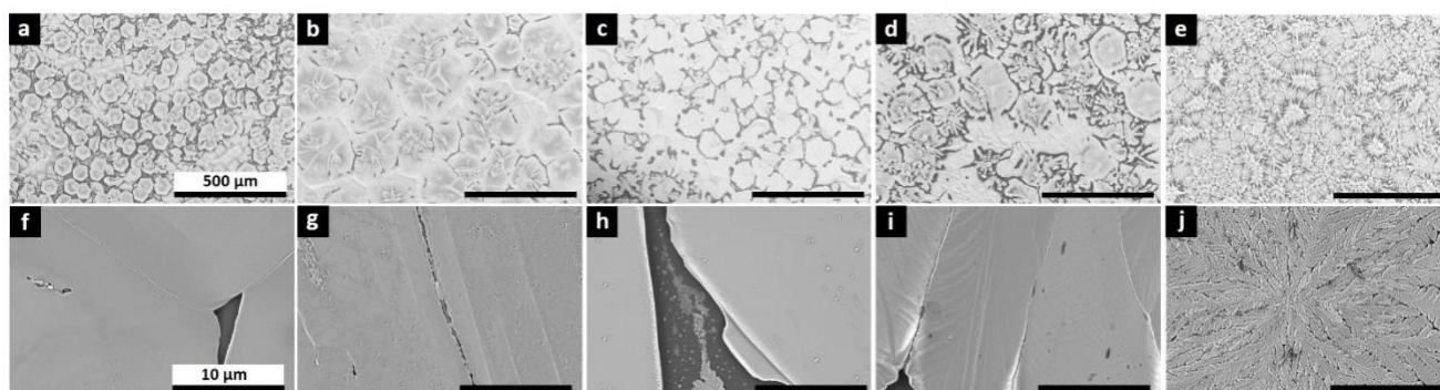
Fig. 2 SEM images of MAPb 0.5 Sn 0.5 I 3 with 0% (a ; f), 0.1% (b ; g), 0.2% (c ; h), 1% (d ; i) and 5% (e ; j) F4TCNQ dopant, using an Everhart-Thornley detector with 100x magnification (a to e) and a Trinity detector with 5000x magnification collecting mostly secondary electrons (f to j). The scale bar is 500 μm for (a) to (e) and 10 μm for (f) to (j).
