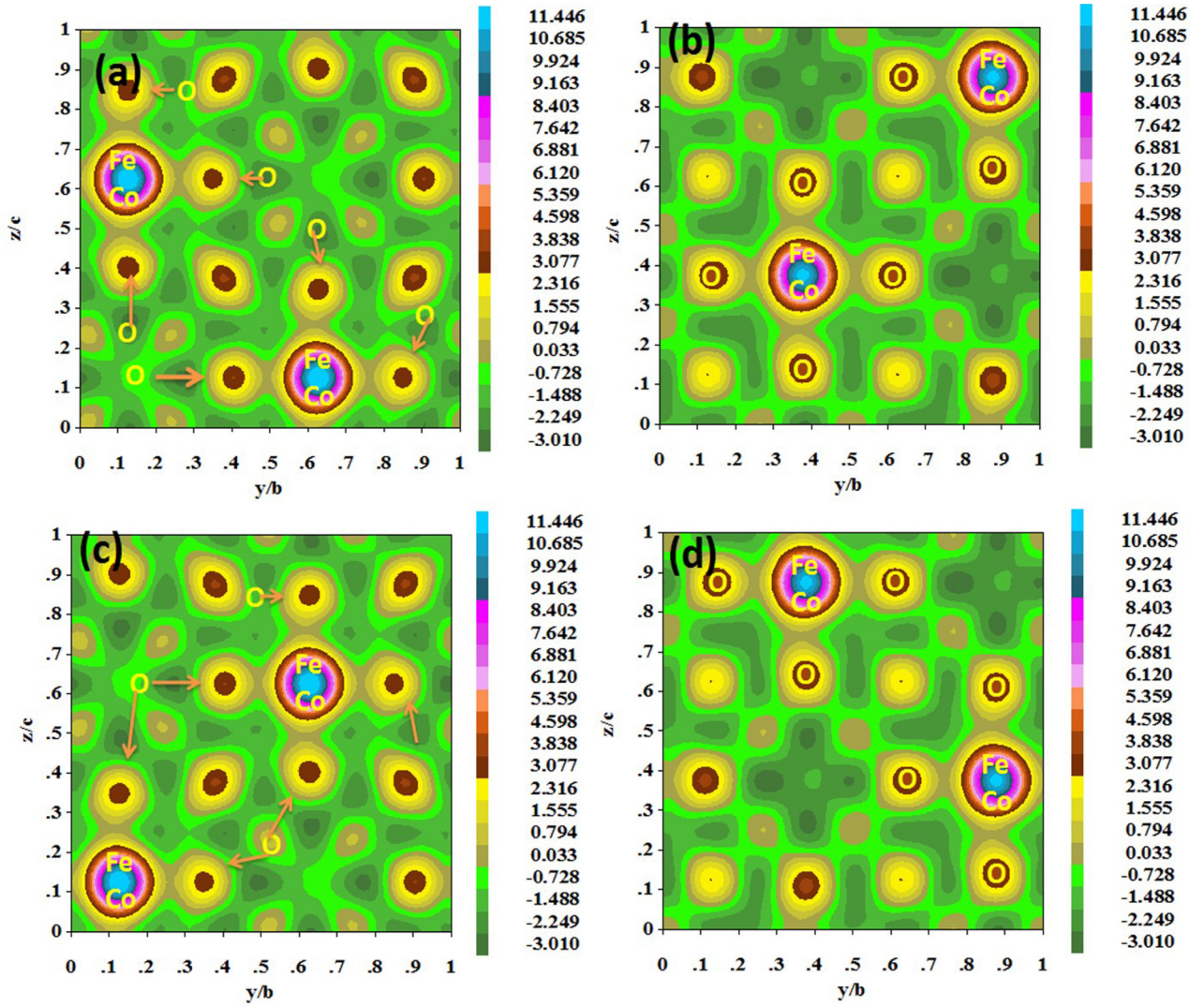
FIG. 6. The electron density (ED) plots in the yz plane taken at the x intercept of x = 0.125 (a), x = 0.375 (b), x = 0.625 (c), and x = 0.875 (d) for CF2.
