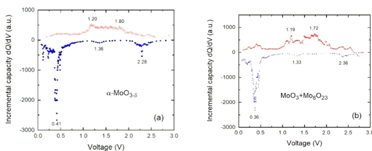
Figure 11. Incremental capacity curves ( dQ/dV ) vs. V of the first lithiation-delithiation cycle for (a) \alpha\text{-MoO}_{3-\delta} and (b) 0.85\text{Mo}_8\text{O}_{23}\text{-}0.15\text{MoO}_3 thin film.
