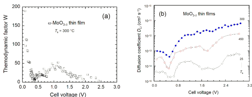
Figure 15. (a) Typical curve W vs. E for a \alpha\text{-MoO}_3 thin film. (b) Apparent \text{Li}^+ ion diffusion coefficients vs. cell voltage determined from PITT measurements for a- \text{MoO}_3 , \alpha\text{-MoO}_3 and 0.85\text{Mo}_8\text{O}_{23}\text{-}0.15\text{MoO}_3 thin films deposited at 25, 300 and 450 °C, respectively.
