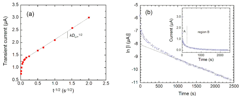
Figure 14. Time-dependent transient current showing the typical potentiostatic intermittent titration technique (PITT) response for PLD \alpha - MoO_{3-\delta} films, (a) at short time ( \tau \ll L^2/D_{Li} ) and (b) at long time ( \tau \gg L^2/D_{Li} ).
