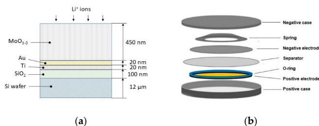
Figure 3. Schematic representation of (a) the cross-sectional view of the \text{MoO}_{3-\delta} thin film electrode deposited on the multilayer substrate and (b) the modified CR2477-type coin cell.
