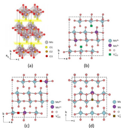
Figure 1. Crystal structure of the layered \alpha - \text{MoO}_3 phase (a) and the vacancies of the three inequivalent oxygen positions O1 (apical) (b), O2 (corner-sharing) (c) and O3 (edge-sharing) (d). Adapted from [20]. Copyright 2016 American Chemical Society.
