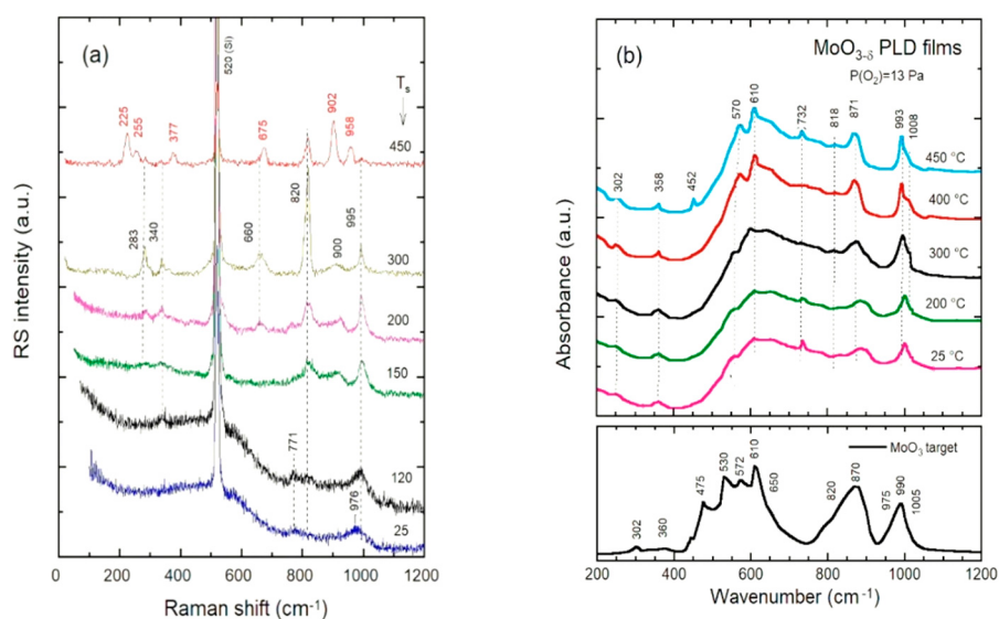
Figure 5. Vibrational spectra of PLD \text{MoO}_{3-\delta} thin films deposited at various temperatures. Each spectrum is shifted vertically for clarity. (a) Raman scattering spectra collected with the laser excitation wavelength of 632.3 nm. Frequencies marked in red are those of \text{Mo}_8\text{O}_{23} . (b) FTIR spectra of \text{MoO}_{3-\delta} thin films and \text{MoO}_3 target (bottom).
