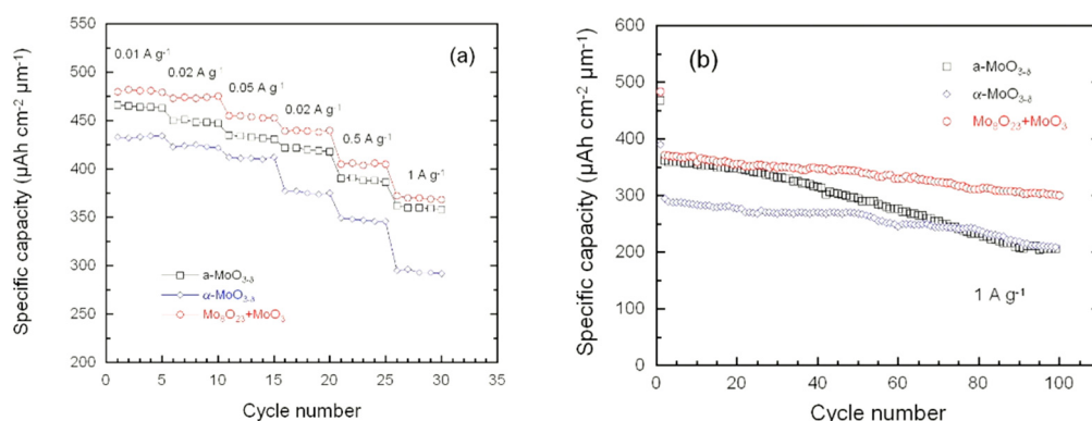
Figure 12. (a) Rate capability and (b) cyclability of MoO 3-δ film in Li cells with 1 mol L −1 LiPF 6 dissolved in ethylene carbonate and dimethyl carbonate (EC:DMC; 1:1 w/w) as aprotic electrolyte.
