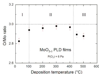
Figure 7. Variation of the O/Mo ratio as a function of the deposition temperature.
