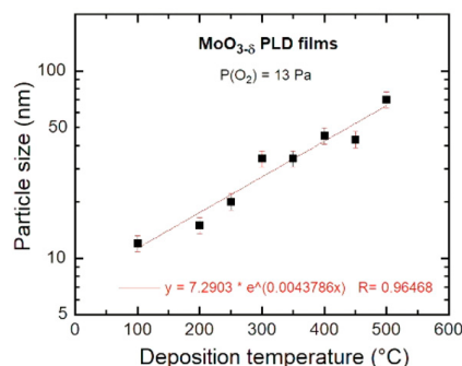
Figure 9. Particle size of \text{MoO}_{3-\delta} films as a function of the deposition temperature.
