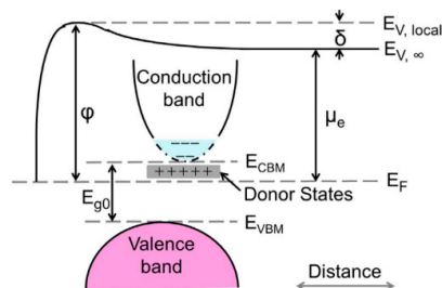
Figure 16. Band structure diagram near the \text{MoO}_{3-\delta} film surface. E_F , E_{g0} , E_{CBM} , E_{VBm} , \phi , \mu_e , E_{V,local} and E_{V,\infty} represent the Fermi level, intrinsic band gap, conduction band minimum, valence band maximum, work function, electron chemical potential, local vacuum level and absolute vacuum level, respectively. Reproduced with permission from [86]. Copyright 2018 Elsevier.
