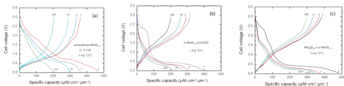
Figure 10. Galvanostatic discharge-charge profiles of \text{Li}^+/\text{Mo-O} thin films recorded at 1 \text{ A g}^{-1} current density in the voltage range 3.0–0.05 V. (a) Amorphous \text{MoO}_{3-\delta} film deposited at 25^\circ\text{C} , (b) \text{MoO}_{3-\delta} film deposited at 200^\circ\text{C} and (c) 0.85\text{Mo}_8\text{O}_{23}-0.15\text{MoO}_3 film deposited at 450^\circ\text{C} .
