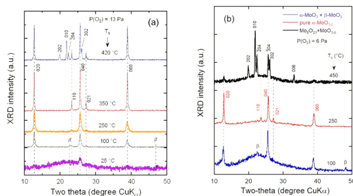
Figure 4. The X-ray diffraction patterns of \text{MoO}_{3-\delta} films deposited using the pulsed layer deposition technique under (a) P_{\text{O}_2} = 13 Pa and (b) P_{\text{O}_2} = 6 Pa. Films were deposited at various substrate temperatures on silicon wafer. Bragg lines have been indexed in the orthorhombic system ( Pbnm S.G.). (0kl) reflections of the \beta - \text{MoO}_3 phase are marked by \beta .
