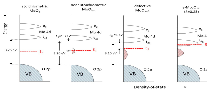
Figure 2. Schematic diagram of the electronic states of molybdenum oxides as a function of the oxygen vacancies. The electronic character varies from insulator ( \text{MoO}_3 , \sigma_e > 10^{-9}\text{ S cm}^{-1} ) to semiconductor (defective \text{Mo}_9\text{O}_{26} , \sigma_e \approx 10^{-2}\text{ S cm}^{-1} ) to metal-like ( \gamma\text{-Mo}_4\text{O}_{11} , \sigma_e \approx 10^4\text{ S cm}^{-1} ).
