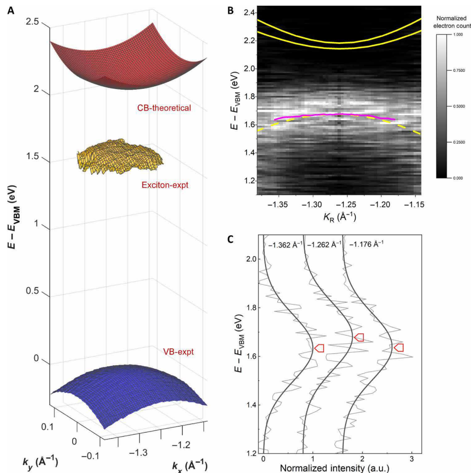
Fig. 3. Anomalous negative dispersion of the electron photoemitted from an exciton. (A) Measured energy-momentum dispersion relationship over the 2D k -space for the electron photoemitted from the exciton and from the VB. Notably, the exciton signal shows a negative dispersion resembling the VB. A theory calculation for the dispersion of the conduction band (CB) is also shown for comparison. The dispersion relationship for the exciton (yellow) and VB (blue) are obtained by fitting the experimental energy distribution curves and extracting their peak values E_X(\mathbf{k}) and E_{VB}(\mathbf{k}) at each momentum. (see Supplementary Text) (B) Measured energy-momentum distribution of the electrons photoemitted from an exciton, along a 1D cut in k -space centered at the K-valley. For each value of k_{||} , the intensity versus the energy is normalized to its maximum value. The yellow solid curves are the theoretical spin-split CBs. The dashed yellow and magenta curves correspond to E_{VB}(\mathbf{k}) and E_X(\mathbf{k}) , with E_{VB}(\mathbf{k}) offset in its energy position for easy comparison to E_X(\mathbf{k}) . (C) Energy distribution curves (light gray) and Gaussian fitting (black) for three representative values of k_{||} from (B), with red \triangle symbol marking the peak positions of the fitted curve.
