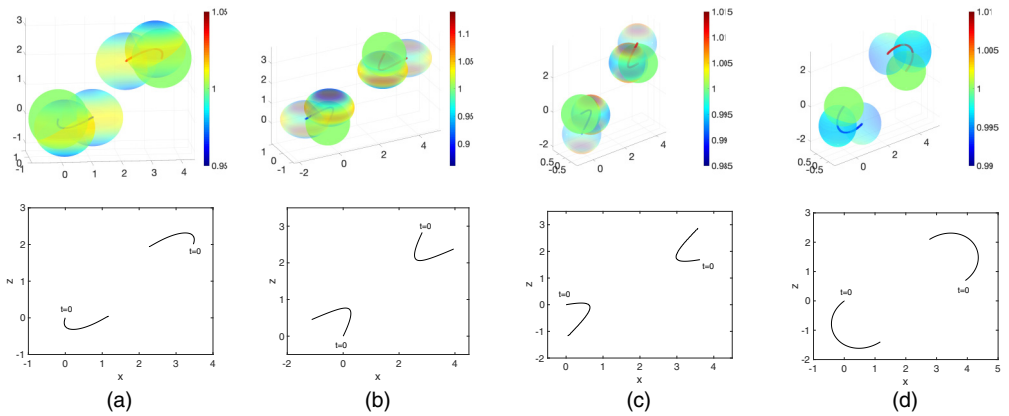
FIG. 7. Trajectories of two identical surfactant-covered drops with (a) R = 0.1 , S = 1 ; (b) R = 1 , S = 10 ; (c) R = 1 , S = 0.1 ; and (d) R = 100 , S = 1 . Initially the drops are in the xz plane, the separation in all cases is d = 4 , and the angle with the applied field direction is (a) \Theta = 60^\circ , (b) \Theta = 45^\circ , (c) \Theta = 65^\circ , and (d) \Theta = 80^\circ . \text{Ca} = 0.1 , E = 1 , and \text{Pe} = 10^6 . Bottom: trajectories in the xz planes. The color map shows the surfactant concentration
