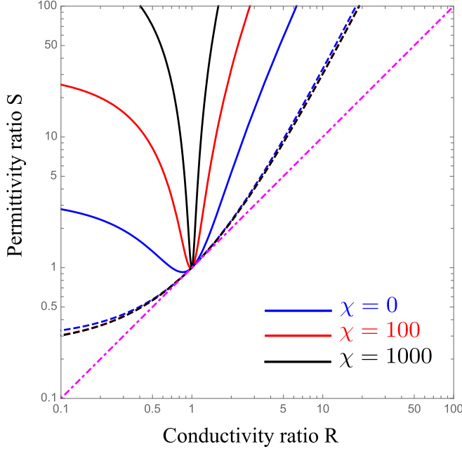
FIG. 2. (a) Phase diagram of drop deformations and alignment with the field for viscosity ratio \lambda = 1 and different values of the parameter \chi = \text{PeMa} . The solid lines correspond to \Phi_s(\lambda, R, S, \chi) = 0 given by Eq. (26); in the parameter space above, the line of centers of the two drops rotates away from the applied field direction \Phi < 0 . The dashed lines correspond to the modified Taylor discriminating function Eq. (A6); in the parameter space above it, drop deformation is oblate, and below it, prolate. Above the dot-dashed magenta line S = R , the surface flow is pole-to-equator ( \beta < 0 ), while below this line the surface flow is equator-to-pole ( \beta > 0 ).
