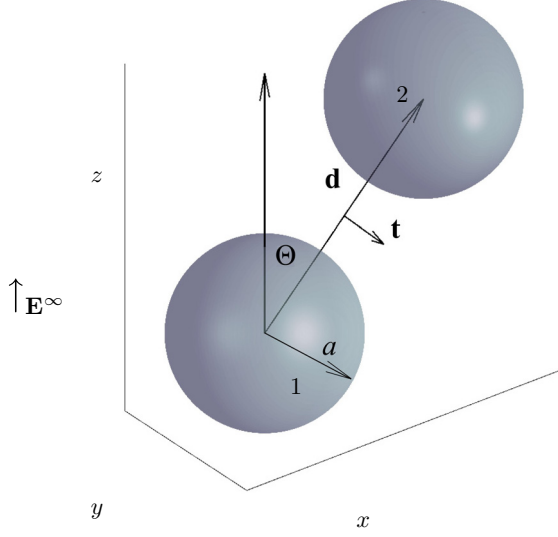
FIG. 1. Two initially spherical identical drops with radius a , permittivity \varepsilon_d , and conductivity \sigma_d suspended in a fluid permittivity \varepsilon_s and conductivity \sigma_s and subjected to a uniform dc electric field \mathbf{E}^\infty = E_0 \hat{\mathbf{z}} . The angle between the line-of-centers vector and the field direction is \Theta = \arccos(\hat{\mathbf{z}} \cdot \hat{\mathbf{d}}) .
