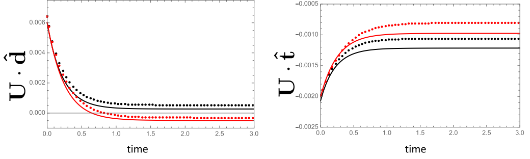
FIG. 6. Evolution of the relative radial (left) and tangential (right) velocities for a drop pair with R = 2 , S = 1 . Initial angle \Theta = 45^\circ and distance d = 4 . Symbols are numerical simulations, and the line is the theory. \chi = 1 (black) and \chi = 10^6 (red). Note that the relative radial velocity changes sign for \chi = 10^6 indicating a change from repulsion to attraction. In both cases, drops move to align their line-of-centers with the applied field direction.
