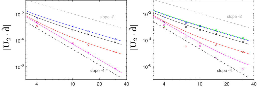
FIG. 3. Steady relative velocity of a pair of leaky dielectric drops aligned with the field ( \Theta = 0 ). R = 2 , S = 1 , Ca = 1 . Left: E = 1 , Pe = 1 (blue); Pe = 10 (black); Pe = 100 (red); and Pe \rightarrow \infty (magenta). The symbols are from our fully 3D code and the solid line is the theory Eq. (25). In the case of nondiffusing surfactant, the interaction is dominated by DEP and the velocity shows 1/d^4 dependence. Right: Pe = 1 and E = 0, 1, 10, 100, 1000 (green, blue, black, red, magenta). As \chi = Ma Pe increases, the critical distance beyond which the DEP dominates increases. Note that \chi = 100 shows a change of slope from -4 and -2 . \chi = 1000 slope -4 in the studied range.
