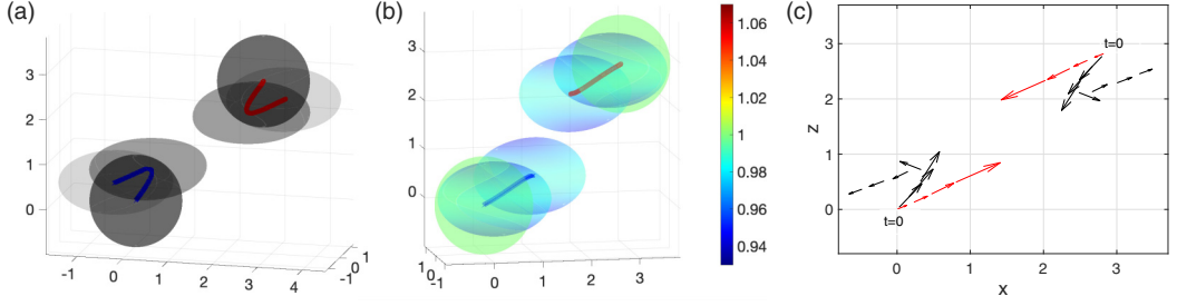
FIG. 5. R = 0.1 , S = 5 , \Theta = 45 . Initial distance d = 4 . (a) Clean drops misaligning, (b) nondiffusing surfactant-covered drops with E = 10 aligning with the field, and (c) center-of-mass trajectory in the x - z plane. Arrows correspond to the velocity for the clean drops (black) and for the nondiffusing surfactant-covered drops (red). See the Supplemental Material [50] for the movies.
