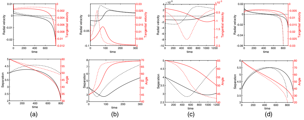
FIG. 8. Dynamics of a pair of identical drops with initial separation d = 4 and different angles with the applied field. Comparison between clean (dotted line) and surfactant-covered drops (solid line) with E = 1 and Pe = 10^6 . Ca = 0.1 . (a) R = 0.1 , S = 1 (repulsion-attraction, alignment with the field); (b) R = 1 , S = 10 (attraction-repulsion, misalignment with the field); (c) R = 1 , S = 0.1 (attraction-repulsion, alignment perpendicular to the field); and (d) R = 100 , S = 1 (repulsion-attraction, alignment with the field).
