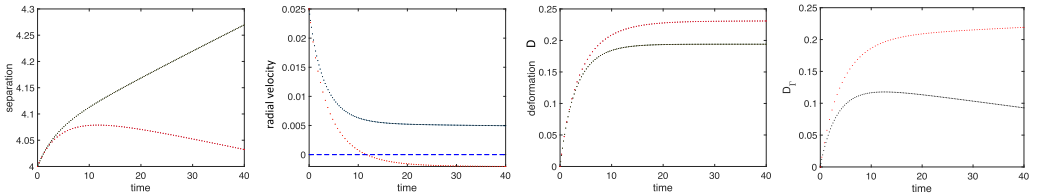
FIG. 4. Effect of surfactant on the interaction of two identical drops with R = 2 , S = 1 , Ca = 1 , E = 1 initially aligned with the field \Theta = 0 . Black dots correspond to Pe = 1 and red dots correspond to the limit of nondiffusing surfactant Pe = 10^6 . The surfactant suppresses the electrohydrodynamic repulsion, and after initial transient due to shape deformation and surfactant redistribution the interaction can reverse sign.
