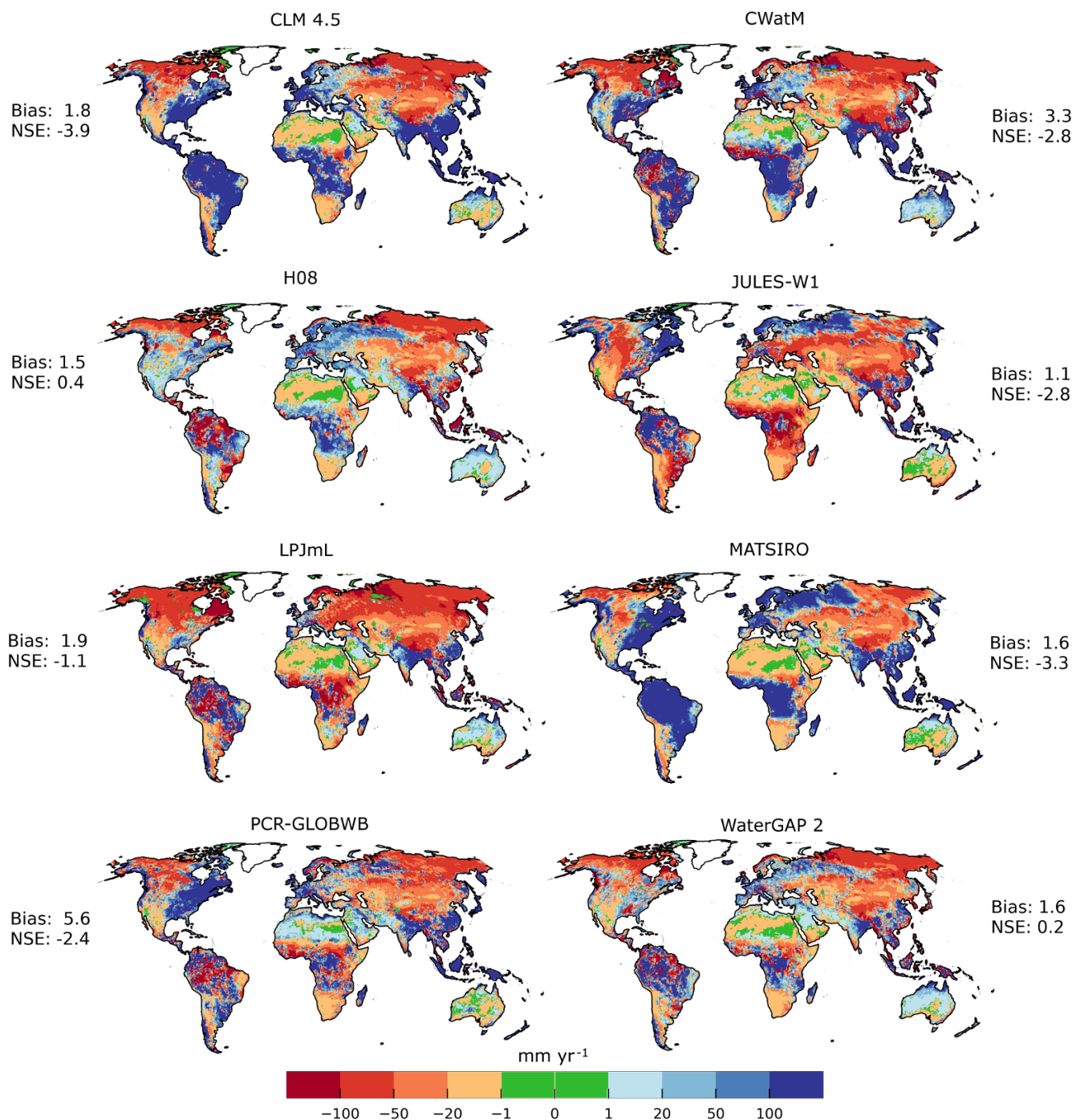
Figure 9. PI GWR per GHM compared to the 34-year (1981–2014) mean GWR ( \text{mm yr}^{-1} ) of Mohan et al. (2018). Bias is the mean (GHM / Mohan et al. 2018). NSE (Nash–Sutcliffe efficiency; Nash and Sutcliffe, 1970) is calculated spatially over all cells instead of time.
