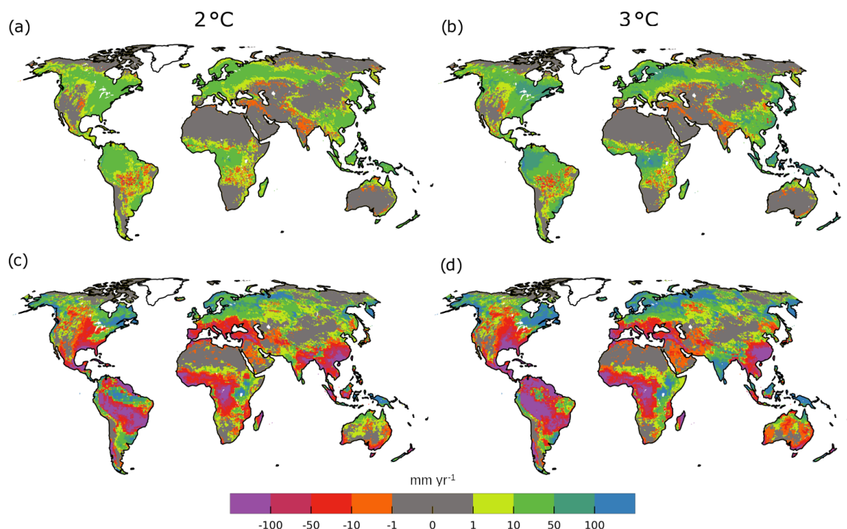
Figure 6. GWR (dynamic \text{CO}_2 ) compared to GWR (static \text{CO}_2 ; \text{mm yr}^{-1} ) for 2.0°C (a) and 3.0°C (b) GW. GWR (dynamic \text{CO}_2 ) compared to PI (dynamic \text{CO}_2 ; \text{mm yr}^{-1} ) for 2.0°C (c) and 3.0°C (d) GW. The figure only includes the GHM CLM 4.5 and the GCM GFDL-ESM2M. Maps show changes in GWR at a certain GW (including all RCPs that lead to that GW with a certain \text{CO}_2 concentration), with dynamically evolving \text{CO}_2 compared to static \text{CO}_2 concentrations from 2005. Green and blue mean that GWR is higher when evolving \text{CO}_2 concentrations are considered; red and purple indicate lower GWR.
