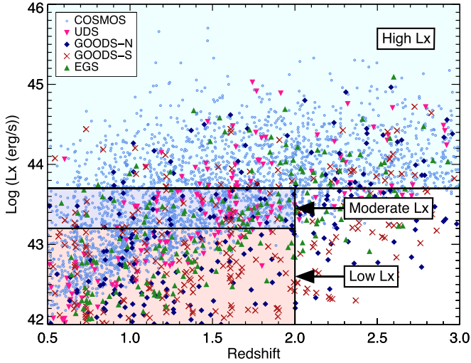
Figure 10. The distribution of the total, i.e., full band (0.5 keV – 10 keV) X-ray luminosity ( L_X ) with respect to redshift for all X-ray AGNs ( L_X > 10^{42} \text{ erg s}^{-1} ) in the COSMOS and CANDELS fields. In the plot, the pink downward triangles, navy diamonds, maroon crosses, green upward triangles, and small light blue circles correspond to all X-ray AGNs in UDS, GOODS-N, GOODS-S, EGS, and COSMOS, respectively. Highlighted are the three L_X - z bins used in our analysis. The light red shaded region (Low L_X bin) show X-ray sources with 42.0 < \log(L_X) < 43.2 at 0.5 < z < 2.0 in the GOODS fields. The lavender (Moderate L_X : 43.2 < \log(L_X) < 43.7 ) and light blue shaded (High L_X : 43.7 < \log(L_X) ) regions correspond to sources in all the fields with 0 < z < 2 and 0 < z < 3 , respectively.
