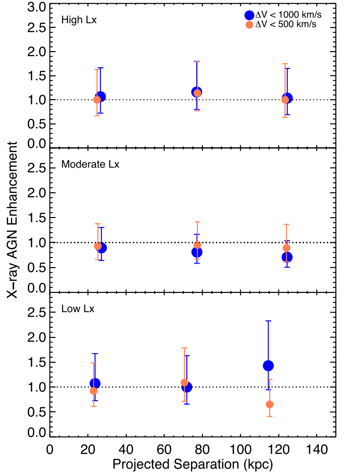
Figure 11. The X-ray AGN enhancement as a function of the projected separation of the paired galaxies with \Delta V < 1000 \text{ km s}^{-1} (large filled blue circles) and \Delta V < 500 \text{ km s}^{-1} (small filled orange circles), split into three different L_X - z bins. The lower panel (Low L_X bin) corresponds to the galaxies in the GOODS-North and GOODS-South fields with 0.5 < z < 2.0 and 42.0 < \log(L_X) < 43.2 . The middle panel (Moderate L_X bin) corresponds to the galaxies in all fields (CANDELS and the full COSMOS field) with 0.5 < z < 2.0 and 43.2 < \log(L_X) < 43.7 . The upper panel (High L_X bin) corresponds to galaxies in all the fields with 0.5 < z < 3.0 and 43.7 < \log(L_X) . The values of the luminosity cut at a given redshift are chosen based on X-ray completeness. The symbols for the pair sample match those in the left panel of Figure 9. The L_X - z bins are defined in Table 4 and illustrated in Figure 10.
