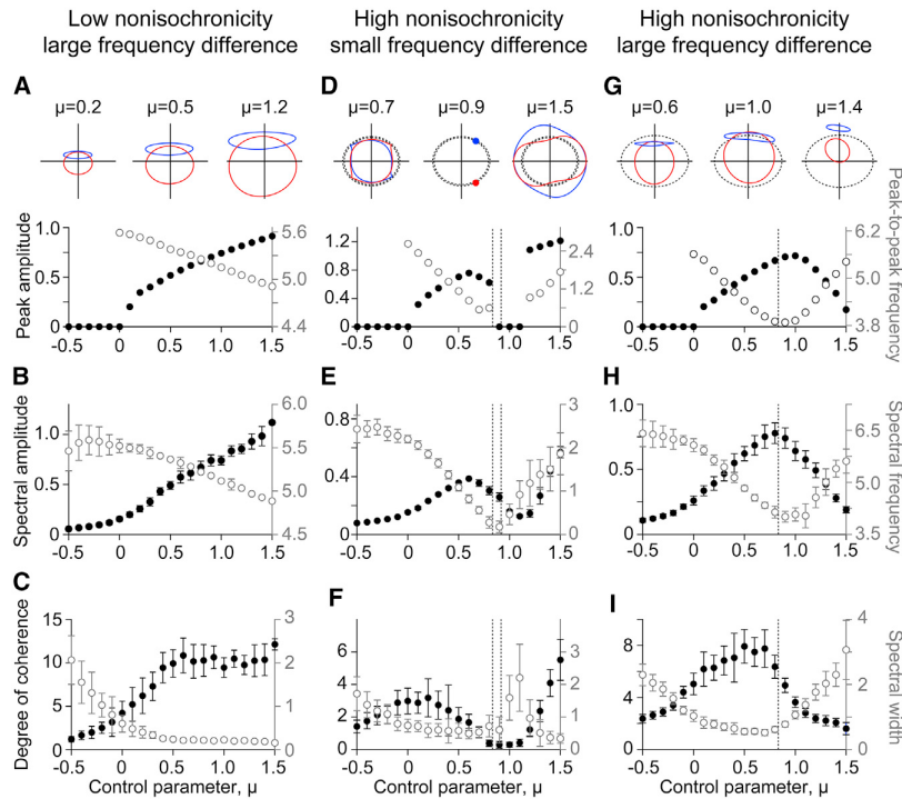
in the vicinity of the angular nullclines (dashed lines). (E) With random fluctuations, the system exhibits tuned behavior. (F) The coherence becomes minimal over a range of the control parameter coinciding with diminishing amplitude. In conjunction with this, the spectral peak reaches a maximum. In (G)–(I), \beta = 3 and \omega_{0,2} = 7.5 . The vertical dashed line indicates the control parameter at the angular nullcline of the first oscillator ( \mu_{0,1} = 0.83 ). (G) In the deterministic limit, strongly nonisochronous oscillators with a large frequency difference show a peak in the spectral amplitude and a minimum in the frequency near the angular nullcline. (Inset) The limit cycles separate in association with the reduction of the oscillation amplitude, as the control parameter exceeds the value at the angular nullcline. (H) Qualitatively similar behaviors are observed upon addition of noise. (I) The degree of coherence exhibits a peak near the maximal spectral amplitude. Within the same range of the control parameter, the width of the spectral peak reaches a minimum.
