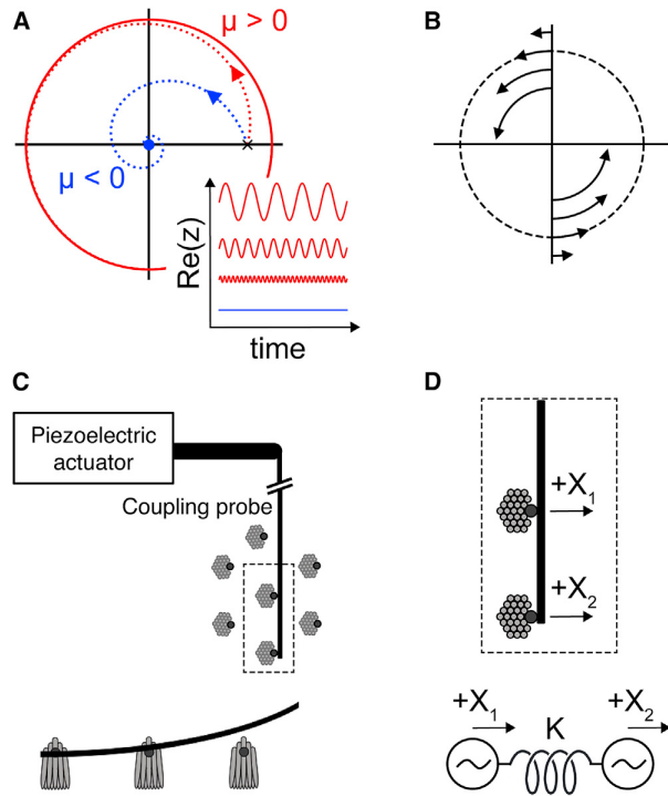
FIGURE 1 The complex displacement, z(t) , of a single, nonisochronous oscillator is described by dz(t)/dt = (\mu + i\omega_0)z - (1 + i\beta)|z|^2z , when \beta > 0 . (A) The complex phase plane is constructed by plotting the imaginary against the real component of z(t) . For \mu > 0 , the trajectory originating from an arbitrary point in the phase plane converges to a limit cycle (red line). For \mu < 0 , the trajectory (blue dashed line) terminates at a stable fixed point at the origin (blue dot). (inset) The oscillator's displacement is stationary for \mu < 0 (blue line) and oscillatory for \mu > 0 (red lines). From bottom to top, the oscillation amplitude increases with \mu , whereas the frequency declines. (B) The complex phase plane illustrates the frequency-amplitude coupling of the nonisochronous oscillator for \beta > 0 . Over a time interval, the trajectory at a higher value of \mu traverses a shorter distance along the limit cycle than that with a smaller \mu . This is associated with the decline in the angular velocity as the amplitude increases. (C) A schematic drawing depicts the glass fiber, with the tip of the coupling probe attached to two hair bundles in the planar epithelium of the bullfrog sacculus, observed from the top-down view of the epithelium. A side view diagram illustrates the curvature of the coupling probe that allows us to avoid contacting other nearby hair bundles. (D) The motion of each hair bundle is perpendicular to the coupling probe, with the positive direction pointing toward the kinociliary bulbs and the attachment point to the probe. The probe-bundles system is modeled as two autonomous oscillators coupled via an elastic element. To see this figure in color, go online.
