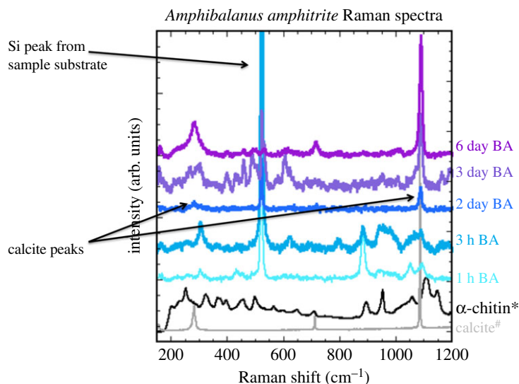
Figure 4. Raman spectroscopy of barnacles at different developmental stages indicates mineralization occurs when the barnacle is between 3 h and 2 days old. The 1 h (light teal) and 3 h old barnacle spectra (light blue) contain peaks consistent with chitin [24] and other organics, while calcitic (light grey [23]) peaks appear in the 2 day (blue), 3 day (light purple) and 6 day old (dark purple) exoskeletons. No amorphous calcium carbonate peaks were observed [24,25].
