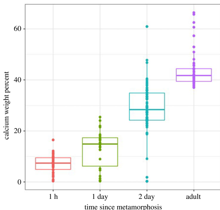
Figure 3. EDS of embedded and polished barnacle parietal plates show a steady increase in calcium content with age. The box-and-whisker plot indicates the median value for each age, with the dark line in the middle of the box, the upper and lower quartiles with the box boundaries, and the outermost measurements with the error bars or whiskers. The amount of calcium within each sample increases as a function of time with the median going from 8% at 1 h old to 16% at 1 day to 28% at 2 days. The adult barnacle had a median value of 44%. Data represent one individual sample per time point, with 26–66 measurements per sample. Graphs of the carbon and oxygen content as a function of time are in the supporting information (electronic supplementary material, figure S5).
