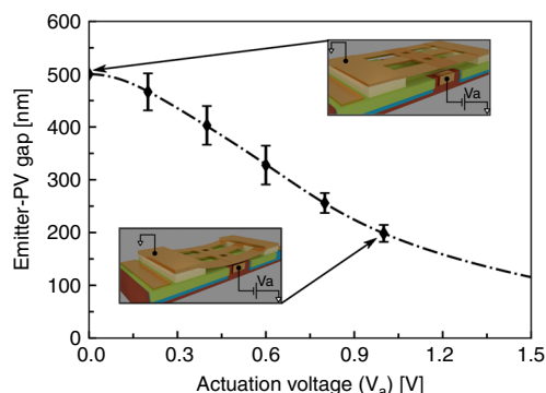
Fig. 3 Nano-electromechanical switch characterization. Displacement of suspended emitter as a function of applied gate-emitter potential difference ( V_a ). The broken line represents fit to a non-linear spring model (see Supplementary Note 7), while the scatter points show the experimental data.
