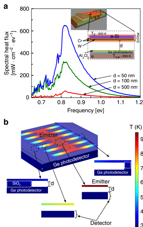
Fig. 2 Computational analysis of near-field heat transfer in our thermo-photovoltaic cell. a Calculated spectral heat flux of thermal radiation absorbed by room-temperature germanium when the hot-emitter (aSi-Cr-W-Cr) is placed at near-field distances (50 nm, blue-line, 100 nm, green line) and, far-away (500 nm, red-line). Inset shows: schematic of the material stack of emitter and photodetector of the thermo-photovoltaic cell. In the hot-stack, chromium (Cr) film helps in adhesion and nucleation of tungsten thin-film, while a-Si provides mechanical support when the bridge is suspended. The cold-stack is composed of Ge-on-silicon and covered with 10 nm alumina ( \text{Al}_2\text{O}_3 ) to protect the surface and avoid any unwanted current leakage from bridge to photodetector in case of shorting during measurement. The temperature of the emitter is assumed to be 900 K. b Simulated temperature distribution in the structure when the emitter is heated up to high temperatures. The insets show the cross-section of the structure at different positions. One can see that the when the emitter is hot (shown by red) the clamped edges at the pad and the substrate remain at room-temperature (shown in blue), due to high-thermal resistance of the thin-film emitter.
