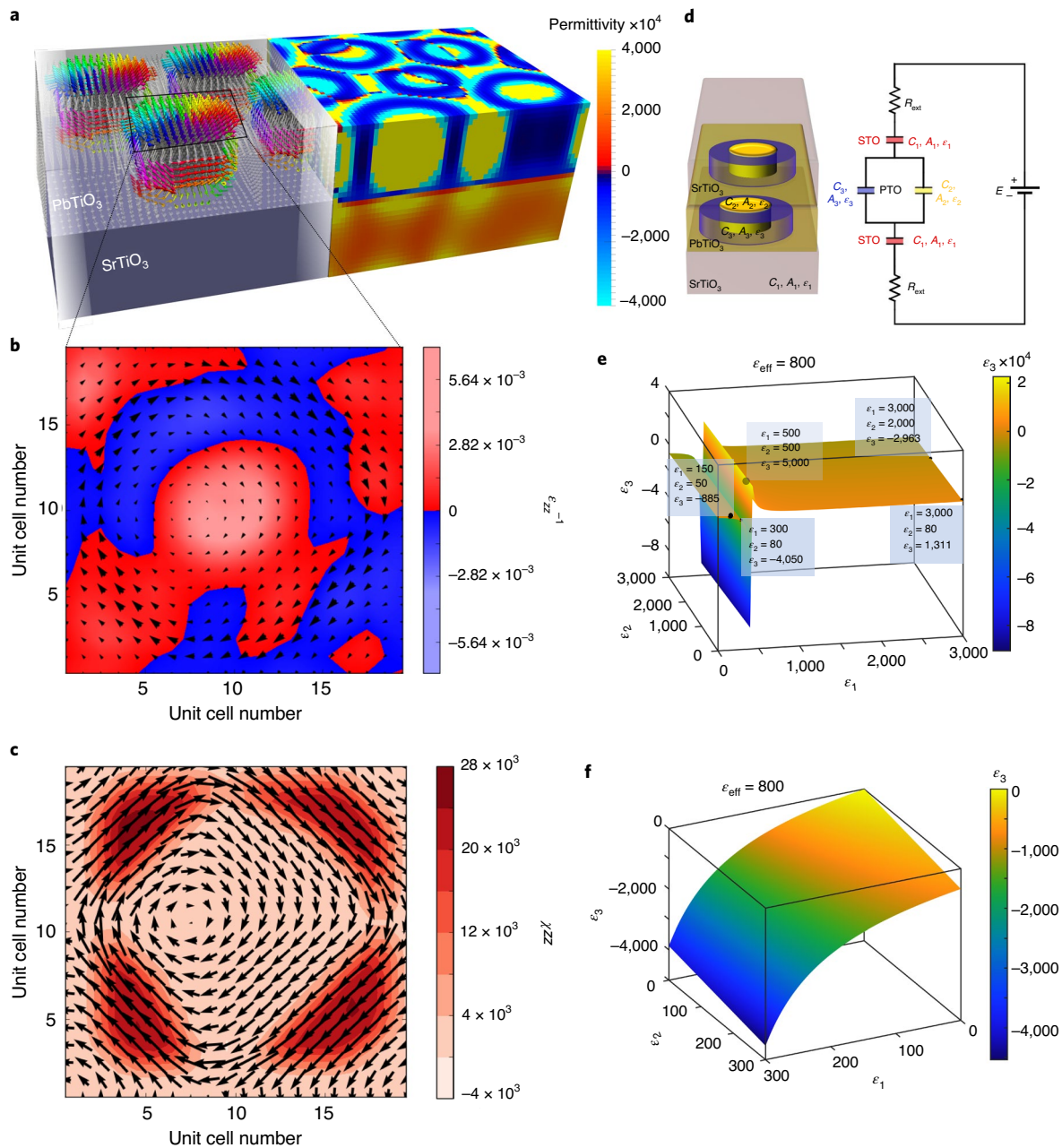
Fig. 2 | Phase-field, second-principles and macroscopic calculations of the negative permittivity of the skyrmion structure at 300 K in a [(SrTiO 3 ) 16 /(PbTiO 3 ) 16 ] 8 superlattice. a , Second-principles calculations of the skyrmion structure (left) and phase-field simulated spatial map of the permittivity of the central PbTiO 3 layer of the skyrmion (right), presenting evidence of local negative permittivity regions (blue contrast). b,c , Second-principles calculations of the two-dimensional distribution of the inverse of the dielectric permittivity ( b ) and the susceptibility at the central plane of PbTiO 3 ( c ) showing the Bloch-like skyrmion texture. Both were computed according to ref. 2 , and the colour codes with key are presented on the right. Both b and c are overlaid by polarization vectors. The arrows represent the components of the polarization in the x-y plane of the skyrmion. d , Macroscopic illustration of our PbTiO 3 /SrTiO 3 system (left, details in Methods) and the corresponding circuit diagram (right). R_{\text{ext}} describes some external resistance of the circuit leading up to the thin-film capacitor, for example, from the electrodes. STO, SrTiO 3 ; PTO, PbTiO 3 . e , Calculations of the permittivity of the skyrmion wall ( \epsilon_3 ) as a function of \epsilon_1 and \epsilon_2 based on the model described in d . A three-dimensional (3D) plot of the interdependence between \epsilon_1 , \epsilon_2 and \epsilon_3 , constrained by an effective dielectric permittivity ( \epsilon_{\text{eff}} ) of 800 (to match the experimental results in Fig. 1a and Supplementary Note 1). The permittivity of the skyrmion wall is always negative except for non-reasonable values of the permittivity of the SrTiO 3 and PbTiO 3 layers, for example, identified by data points with fictitious permittivities. These fictitious scenarios are unlikely because it would mean that both SrTiO 3 and PbTiO 3 have a substantially enhanced permittivity compared with that in the bulk. f , A section of the phase space in e , showing the permittivity of the skyrmion wall ( \epsilon_3 ) as a function of \epsilon_1 and \epsilon_2 specifically for values of SrTiO 3 and PbTiO 3 layer permittivities in the range 0–300 (which is a reasonable range for thin films), showing that the wall permittivity is negative over the entire range.
