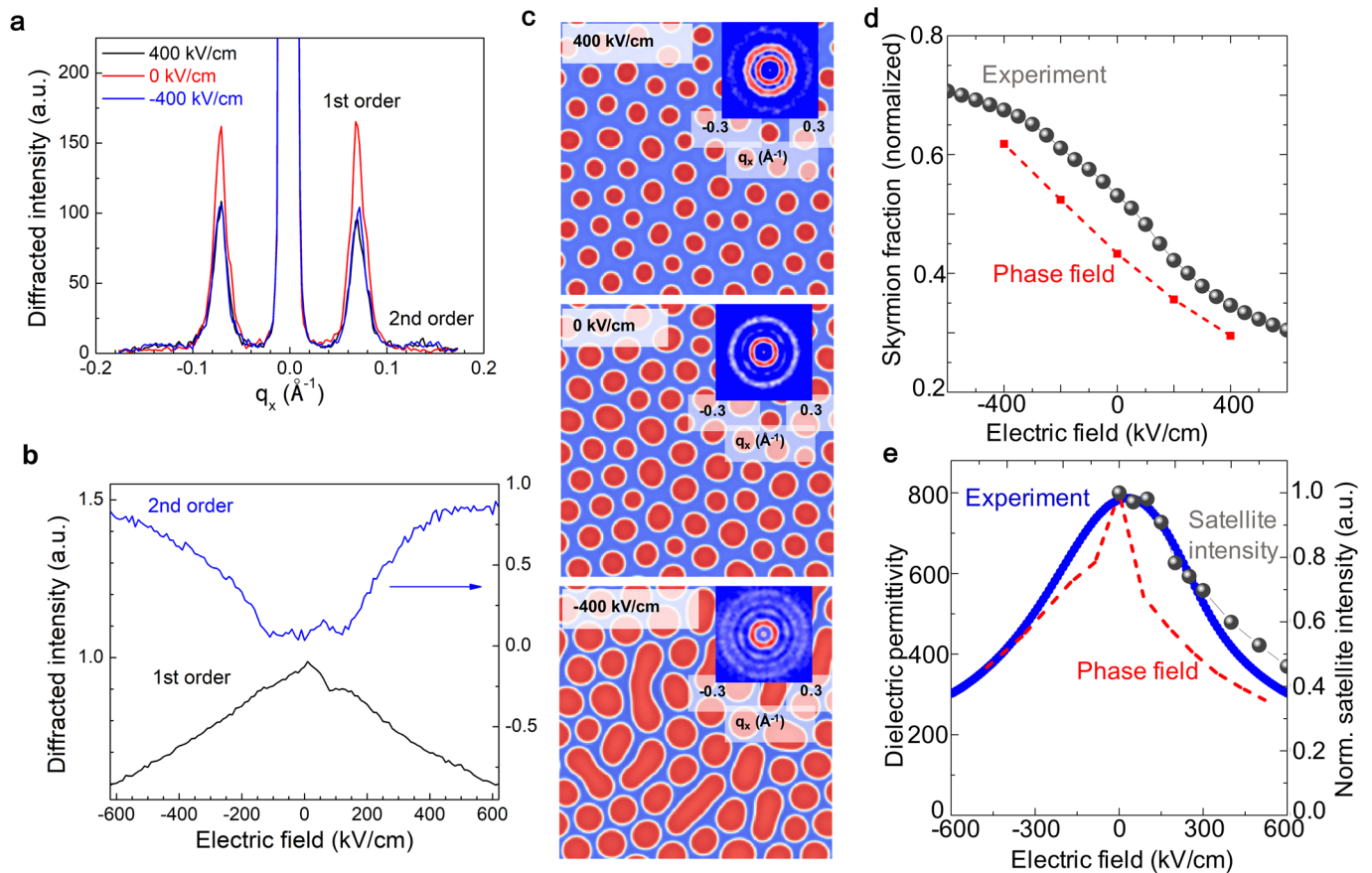
Extended Data Fig. 9 | Tunable skyrmion size under electric field as a basis for dielectric enhancement [(SrTiO 3 ) 16 /(PbTiO 3 ) 8 ] superlattice.
