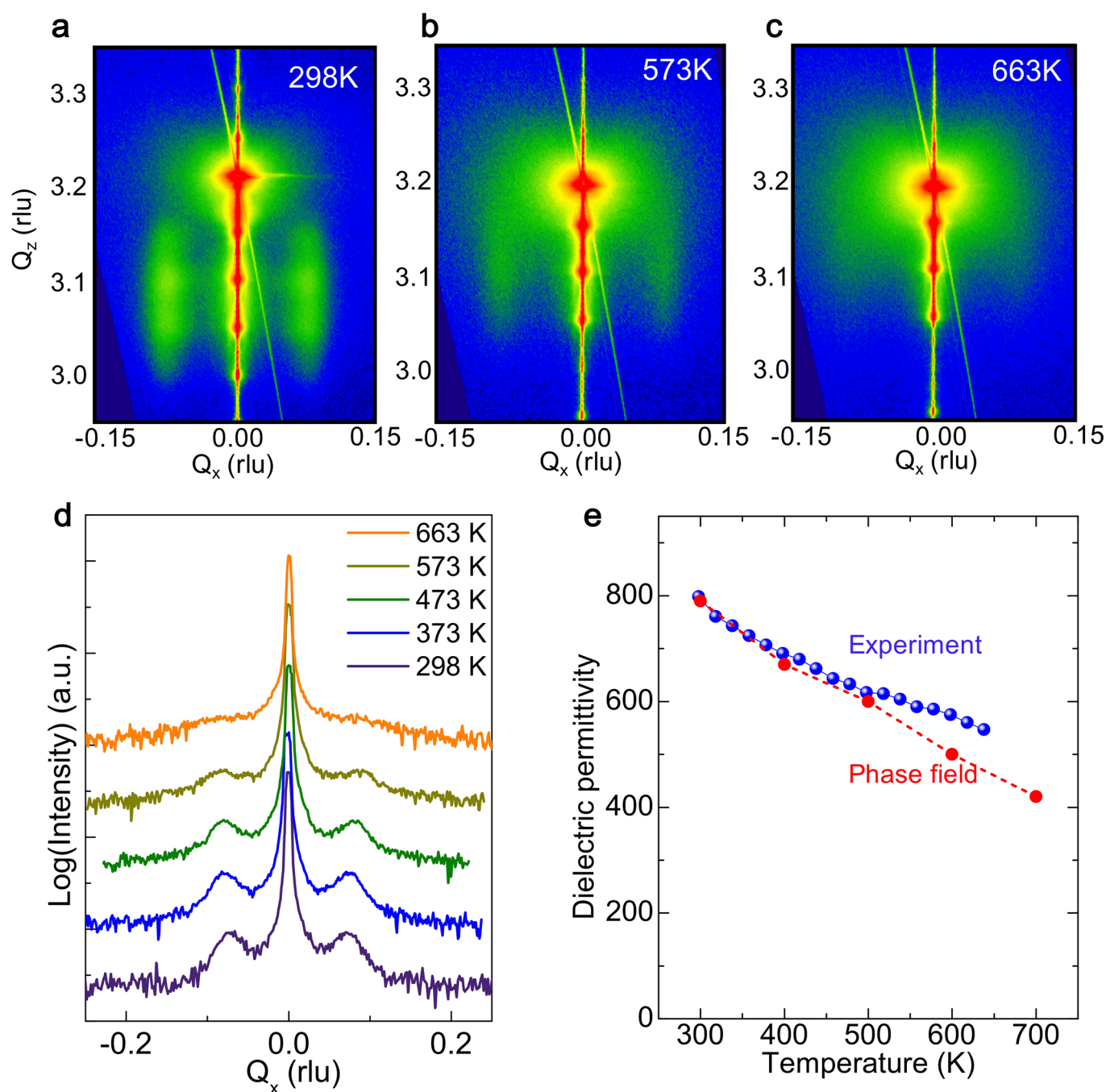
Extended Data Fig. 10 | Temperature control of skyrmion of [(\text{SrTiO}_3)_{16}/(\text{PbTiO}_3)_{16}]_8 superlattice. a-c , Temperature dependent three-dimensional, synchrotron-based symmetric reciprocal space mapping about the (002) diffraction condition of the \text{SrTiO}_3 substrate. The satellite peaks along (100) direction (side-lobes) which correspond to the skyrmions. d , The in-plane satellite peaks intensity (skyrmion peaks) diminishing upon heating and completely disappeared \sim 600\text{K} . e , Comparison between the temperature-dependent experimentally measured and phase-field calculated out-of-plane dielectric permittivity of the superlattice.
