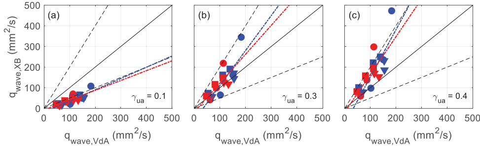
2009) and red (Ruessink et al., 2012) lines. One-to-one correspondence between the two transport rates is shown by the solid-black lines, and the dashed-black lines have slopes one-half and twice the slope of the one-to-one lines. (For interpretation of the references to colour in this figure legend, the reader is referred to the Web version of this article.)
