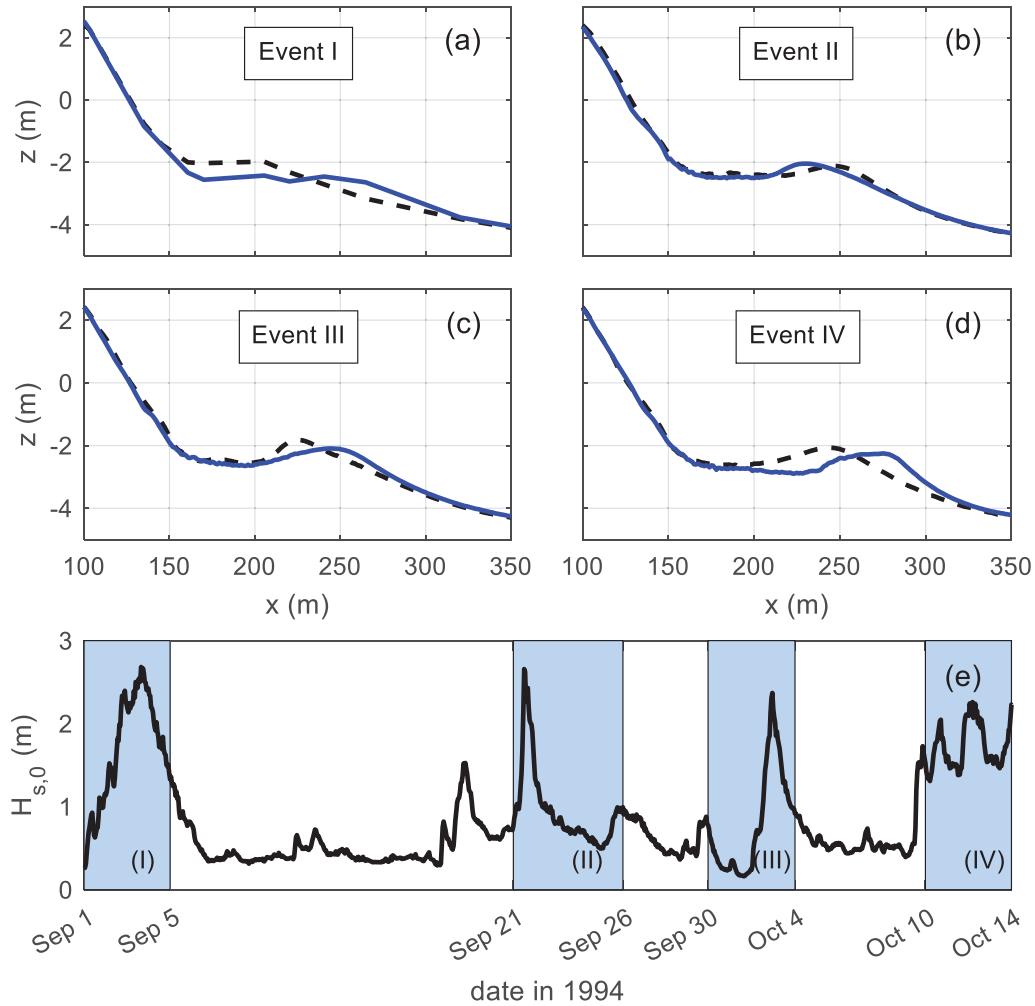
Fig. 2. Seafloor elevation z versus cross-shore location x for (a) Event I (offshore sandbar migration between September 1 (dashed-black curve) and September 5 (solid-blue curve)), (b) Event II (onshore migration between September 21 (dashed-black) and September 26 (solid-blue)), (c) Event III (offshore migration between September 30 (dashed-black) and October 4 (solid-blue)), and (d) Event IV (offshore migration between October 10 (dashed-black) and October 14 (solid-blue)), and (e) hourly averaged significant wave height measured in 8-m water depth H_{s,0} versus date (sandbar migration event dates shaded in blue). (For interpretation of the references to colour in this figure legend, the reader is referred to the Web version of this article.)
