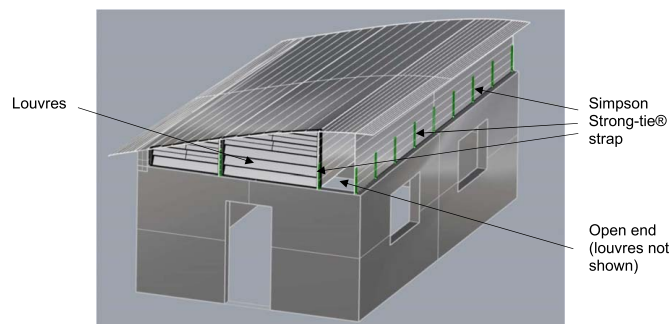
Fig. 4. Schematic of roof.
