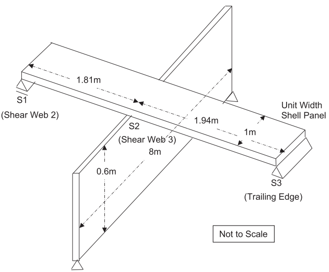
Fig. 6. Analytical model of the shell panel and supports.
