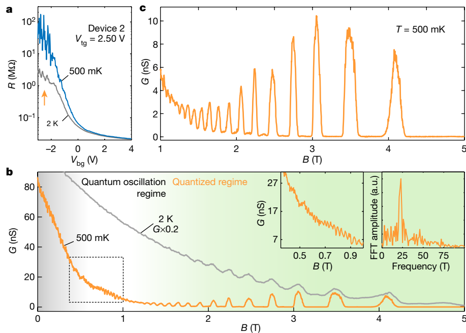
Fig. 3 | Quantized regime and discrete Landau levels in the monolayer insulator. a , Two-probe resistance R , taken from device 2, as a function of V_{bg} ( V_{tg} = 2.5 V). b , Magnetic-field-dependent conductance G , defined as 1/R , taken at a selected gate voltage ( V_{bg} = -2.5 V, indicated by the arrow in a ). Data taken at 500 mK (orange) clearly display the fully quantized regime (shaded with green),
