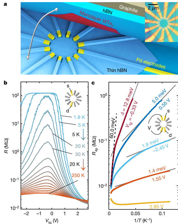
Fig. 1 | Device schematic and the insulating state of monolayer WTe 2 .
