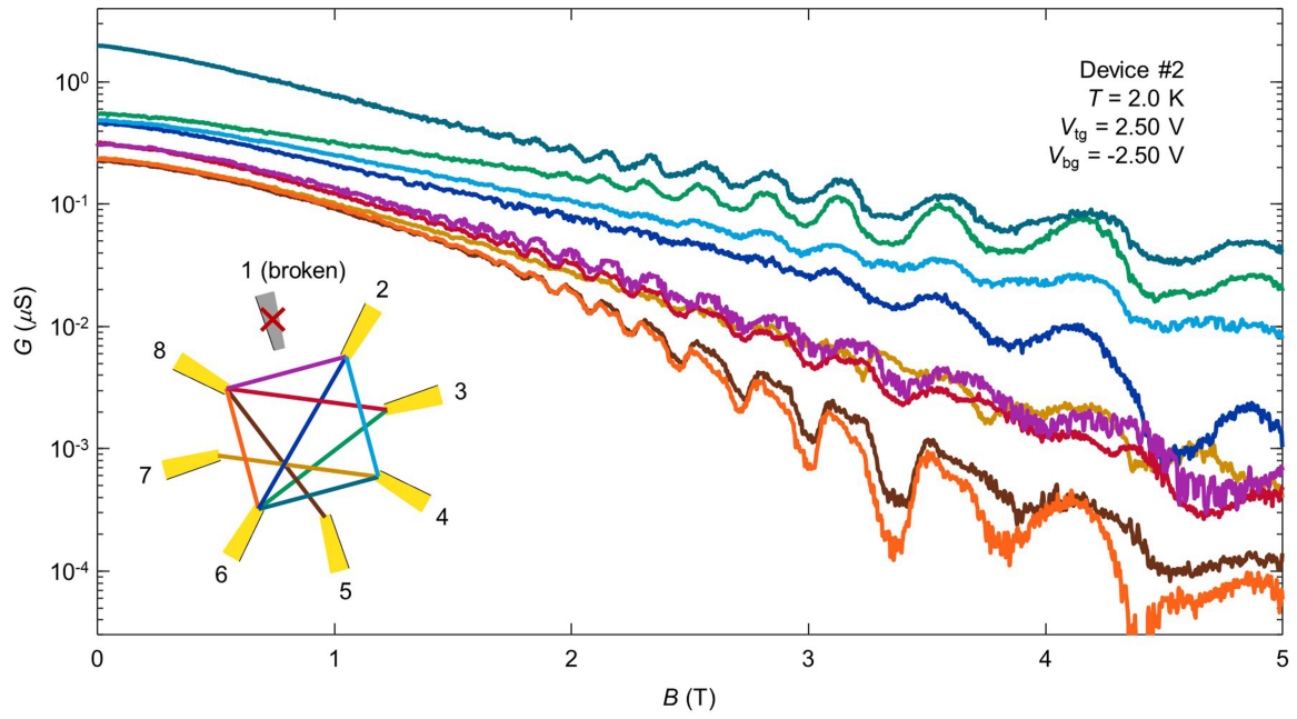
Extended Data Fig. 5 | Quantum oscillations observed when using different contact configurations in device 2. The QOs are robustly observed between various contact pairs connected to the monolayer WTe 2 flake. In this device, 7 out of 8 contacts are working (contact 1 was broken during fabrication). Inset, the contact pairs for each data curve. For each coloured data curve, the source
