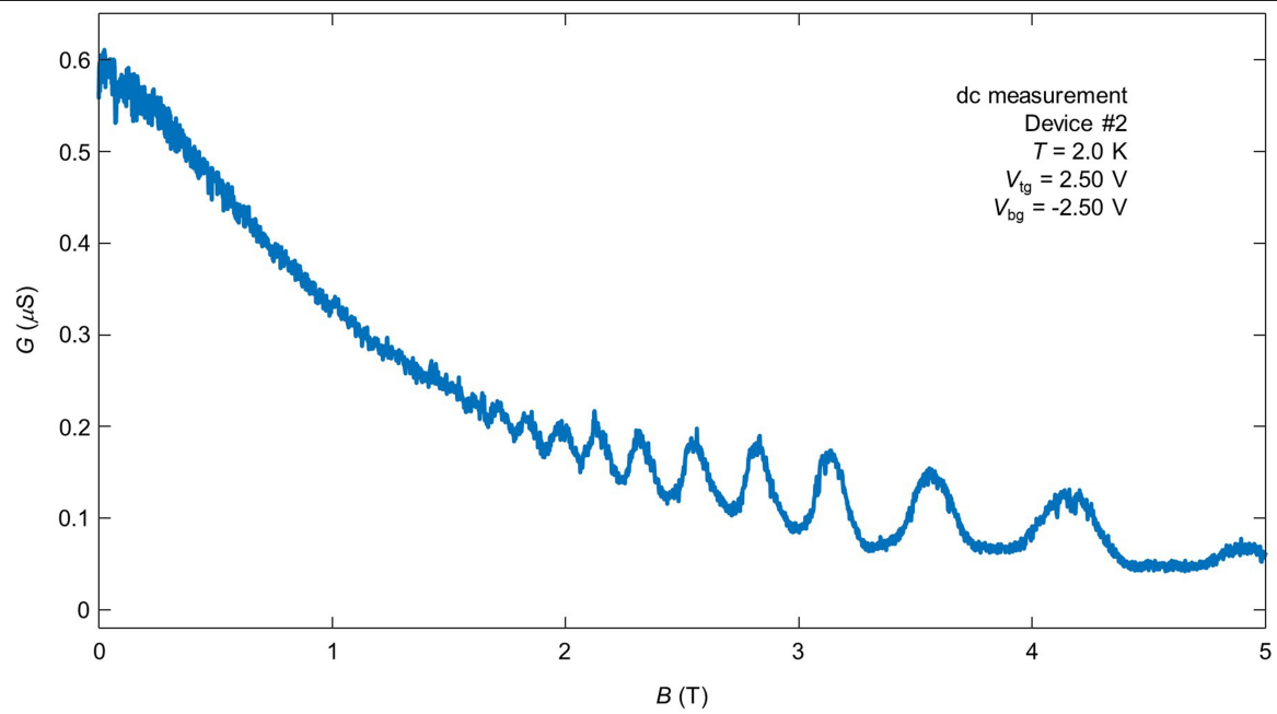
Extended Data Fig. 6 | Quantum oscillations observed in d.c. measurements. The two-probe d.c. conductance ( G ) as a function of the magnetic field B was measured by applying a small d.c. excitation with an amplitude of 1.5 mV via a Keithley 2400 while monitoring the d.c. current.
