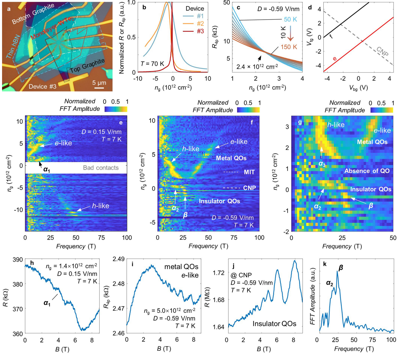
Extended Data Fig. 3 | Quantum oscillations observed in device 3 with high charge-carrier mobility. a , An optical image of device 3. The red dashed line highlights monolayer WTe 2 . b , Comparison of the gate-tuned resistance of the three devices at 70 K (normalized R_{4p} for devices 2 and 3, and normalized R for device 1). See Methods for definition of n_g . c , Gate-tuned R_{4p} of device 3 with a fixed D = -0.59 \text{ V nm}^{-1} ( D \equiv (V_{bg}/d_{bg} - V_{tg}/d_{tg})\epsilon_i/2 ), showing the metal-insulator transition (MIT) at n_g \approx 2.4 \times 10^{12} \text{ cm}^{-2} , indicated by the arrow. d , Schematic diagram of gate-tuning traces used in e (red) and f (black), along which lines D is fixed while n_g is varied. The dashed line indicates the CNP. e , Normalized FFT amplitude of the QOs under varying n_g at D = 0.15 \text{ V nm}^{-1} (see Methods for discussion of D and of the normalization of FFT amplitude). In addition to the
