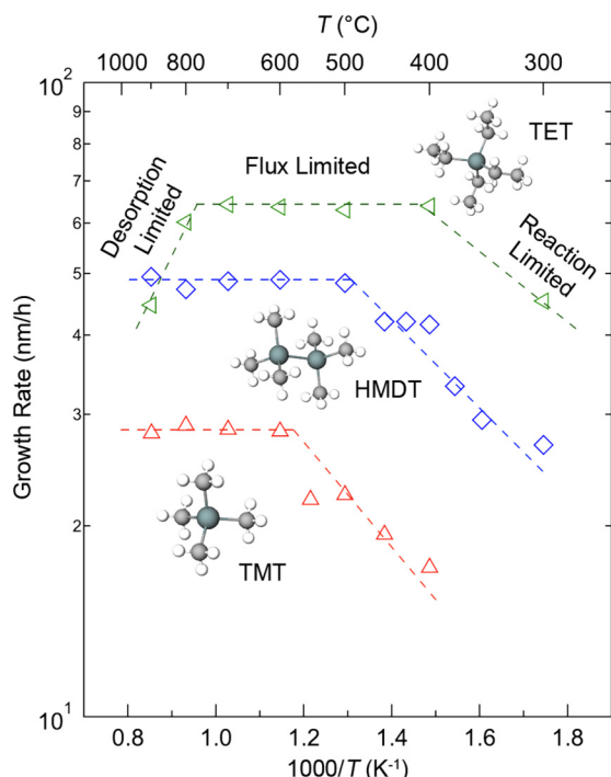
FIG. 3. Growth rates of SnO 2 films on r -Al 2 O 3 (10 \bar{1}2 ) as a function of growth temperature for the three precursors—tetramethyltin (TMT), hexamethylditin (HMDT), and tetraethyltin (TET). All films were grown at a Baratron® setpoint pressure of 140 mTorr. Reaction-limited, flux-limited, and desorption-limited growth regimes are identified. The growth rates for SnO 2 films grown using TET are taken from Wang et al. , J. Vac. Sci. Technol. A 33 , 020606 (2015). Copyright 2015 American Vacuum Society.
