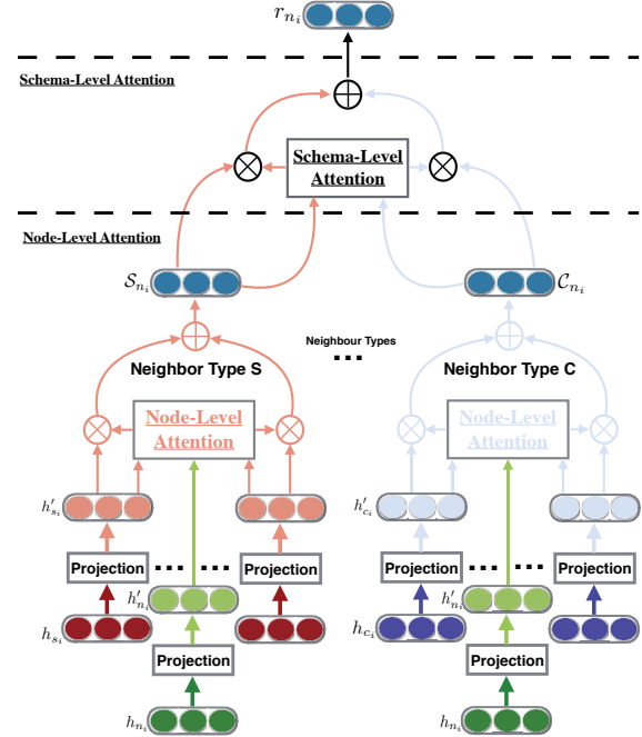
Fig. 3. Hierarchical Graph Attention Neural Network.
