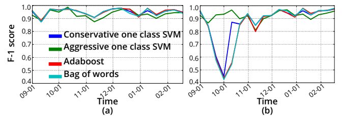
Figure 8: Comparing decider algorithms with: (a) 10 day and (b) 60 day retraining intervals.
