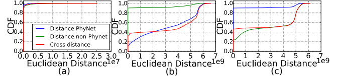
Figure 14: The Euclidean distance (computed over feature vectors) using (a) just the server features, (b) just the switch features, and (c) just the cluster features.
