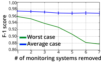
Figure 9: The framework can adapt to deprecated monitoring systems.
