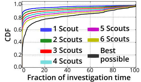
Figure 15: The amount of investigation time we can reduce for mis-routed incidents by adding more Scouts.
