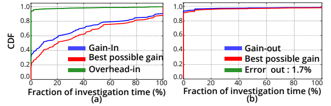
Figure 7: Gain/overhead for mis-routed incidents: (a) gain/overhead in (b) gain/error out.
