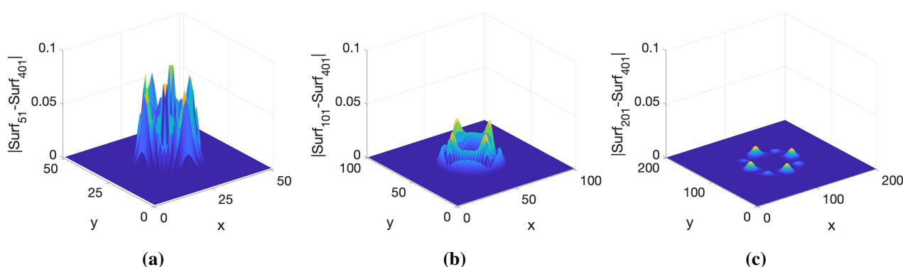
Figure 12. Surface differences. (a). Between N = 51 and N = 401 . (b). Between N = 101 and N = 401 . (c). Between N = 201 and N = 401 .
