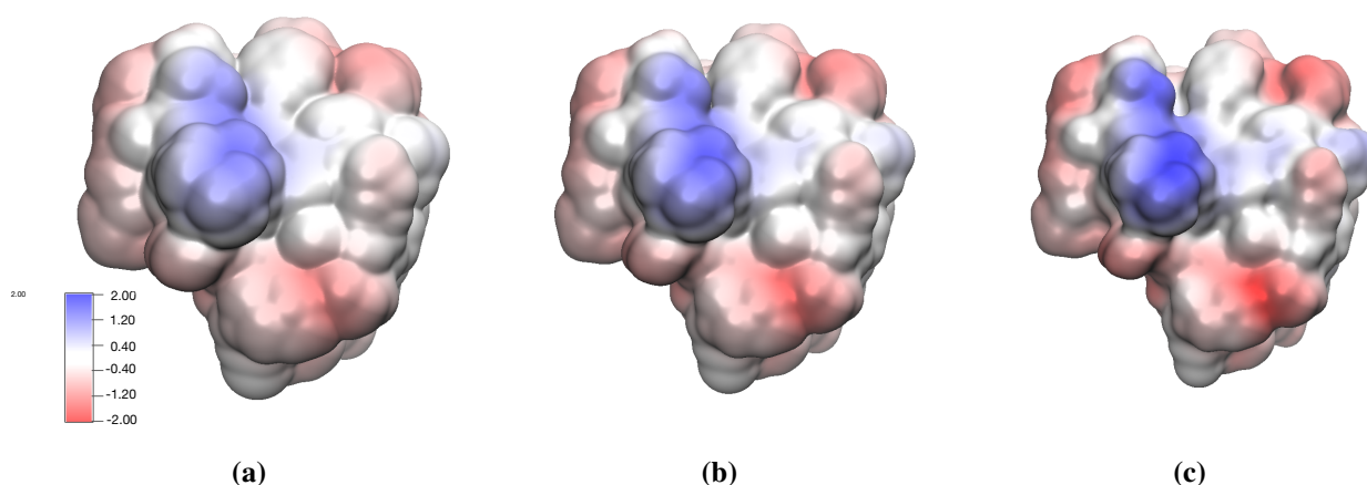
Figure 19. Plots of the surface potentials of the protein 1AHO at different isosurfaces S = \text{const.} (a) S = 0.1 ; (b) S = 0.5 ; (c) S = 0.9 .
