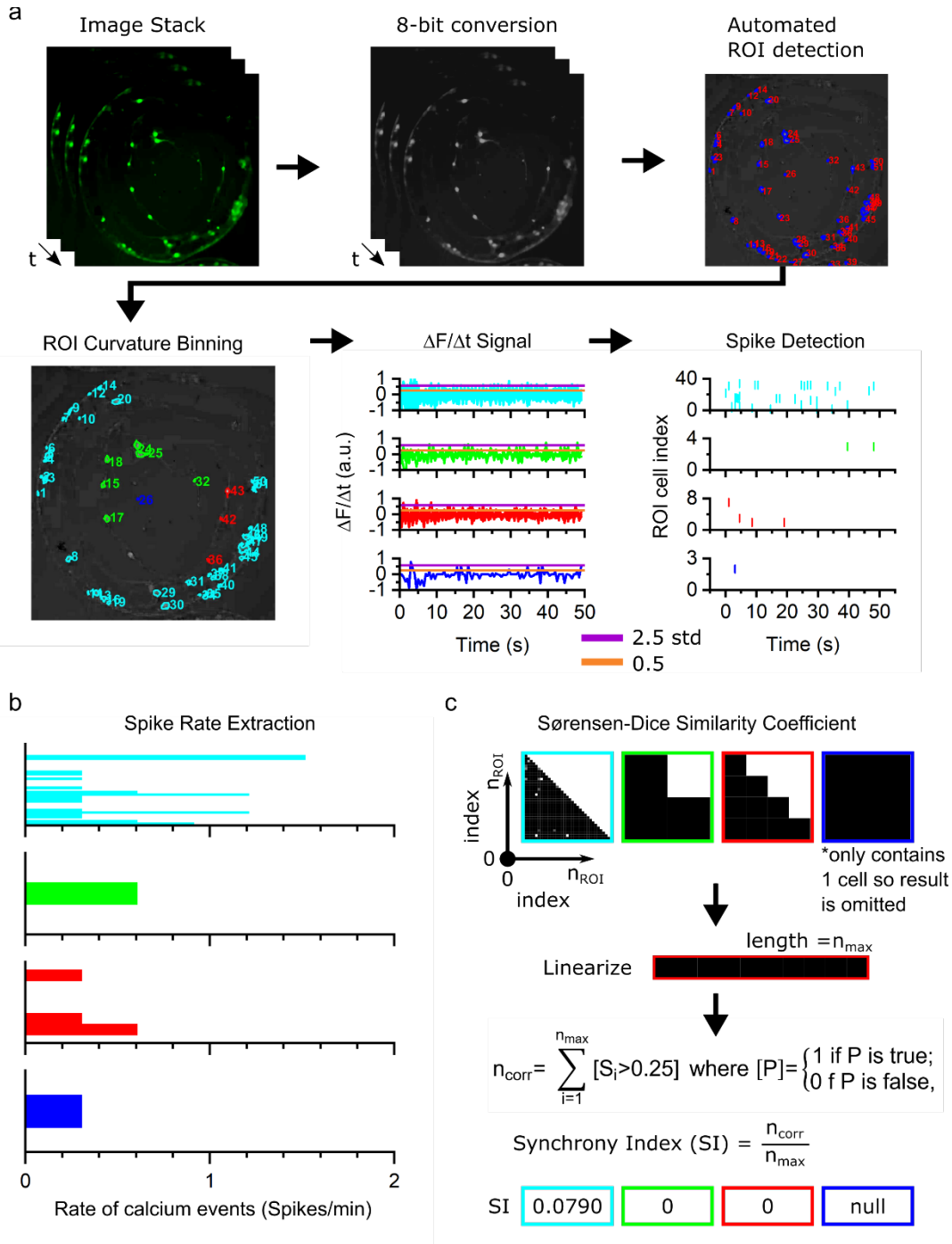
Figure S5: Image processing workflow to extract curvature-dependent transient calcium activity. (a) Selected multi-curvature pattern with temporal changes in fluorescent (12-bit, RGB) gets downsampled to gray-scale (8-bit). Automatic selection of a region of interest (ROI) based on single-cell body ( n_{ROI} ) segmentation is applied and subjected to a curvature mask specific to the pattern. For each specific ROI, changes in calcium fluorescence over time ( \Delta F/\Delta t ) are captured. Spike events based on increasing calcium levels then get detected, and calcium events sorted based on distinct multi-curvature regions. (b) Bar plots show accumulated calcium events based on spike rate per minute associated with the distinct multi-curvature regions. (c) Synchronous calcium event activity within the neuronal network in each distinct curvature region is determined based on a comparison of correlated spikes ( n_{corr} ) over total number of spikes ( n_{max} ) using the Sørensen–Dice similarity coefficient and a synchronicity index (SI).
