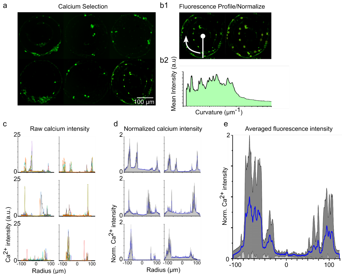
Figure S4: Static calcium ( \text{Ca}^{2+} ) fluorometry for a single multi-curvature pattern. (a) False-color fluorescent image shows a representative sample set of calcium-labeled (Fluo4 AM) neuronal cell growth in the multi-curvature patterns. (b1) A custom semi-automatic script acquires raw fluorescent intensity profiles circulating clockwise through the pattern. (b2) Extracted raw fluorescent intensity profiles showing the mean of all collected surface profiles. (c) Extracted raw mean intensity profiles from six individual patterns of the same topography (15 \mu\text{m} agarose barrier width, 10 \mu\text{m} groove width = curvature region). Intensity values are based on an 8-bit scale (0-255). (d) Normalized calcium intensity plots based on cell count per curvature region and mean intensity. (e) Averaged calcium intensity profiles for the six selected topographically identical micro curvature patterns.
