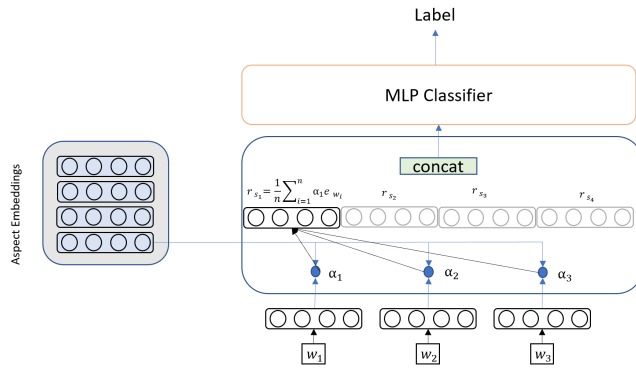
Figure 3: Architecture of attention model
