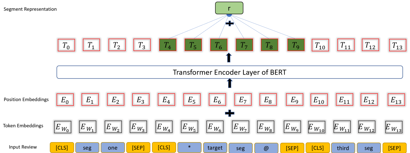
Figure 2: Representation layer
