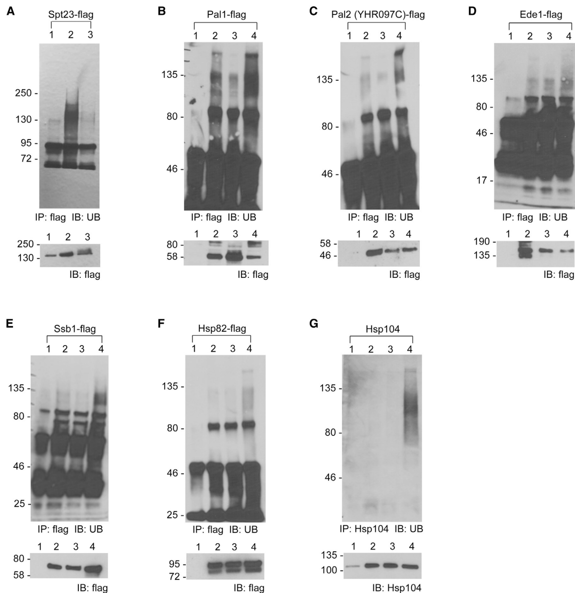
Figure 5. Assaying the Rsp5-catalyzed substrate ubiquitination in cim3-1 cells shifted to 37°C
