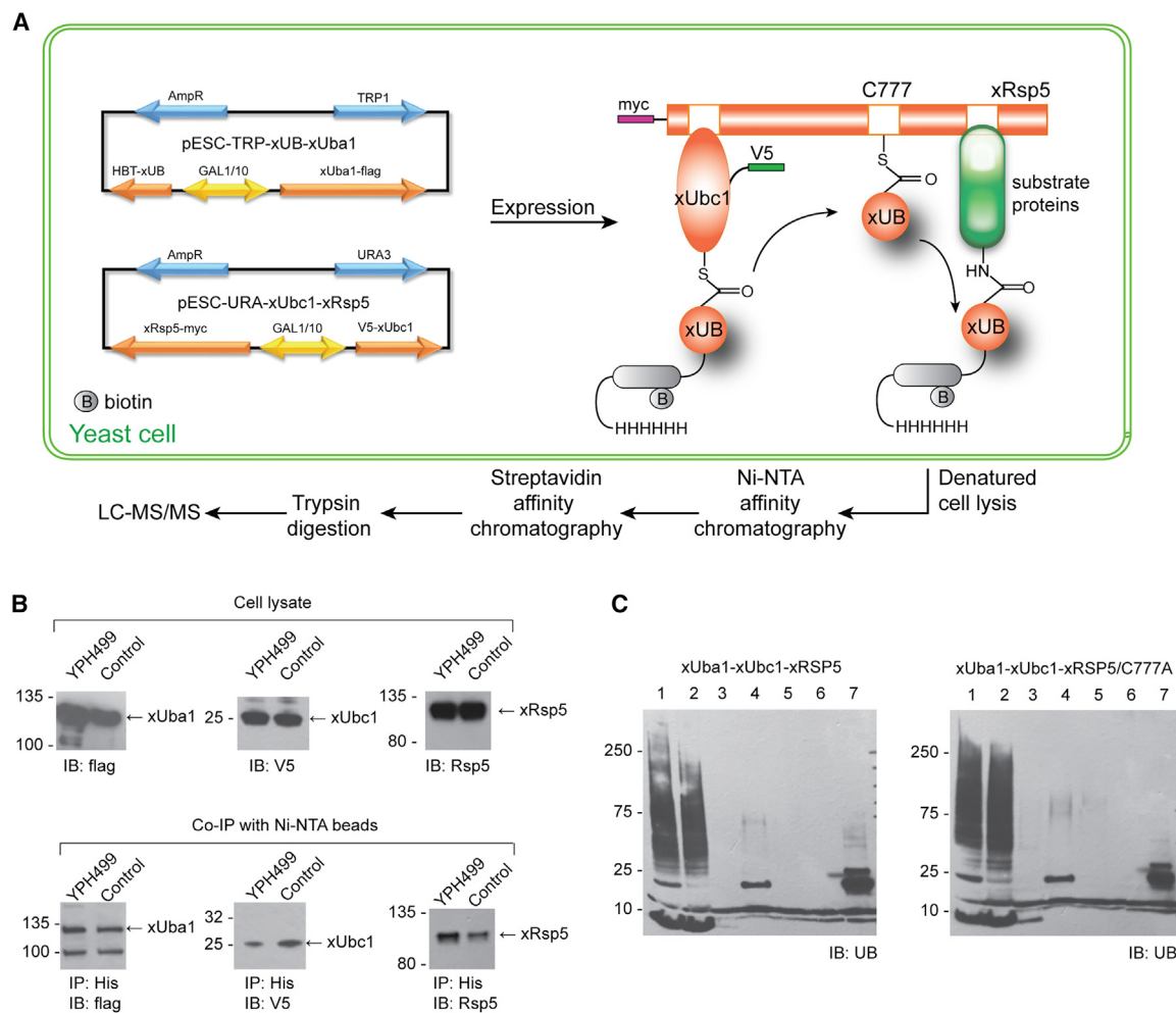
Figure 3. Schematic representation of the outline for the OUT cascade of Rsp5 in yeast cells to profile its substrates
