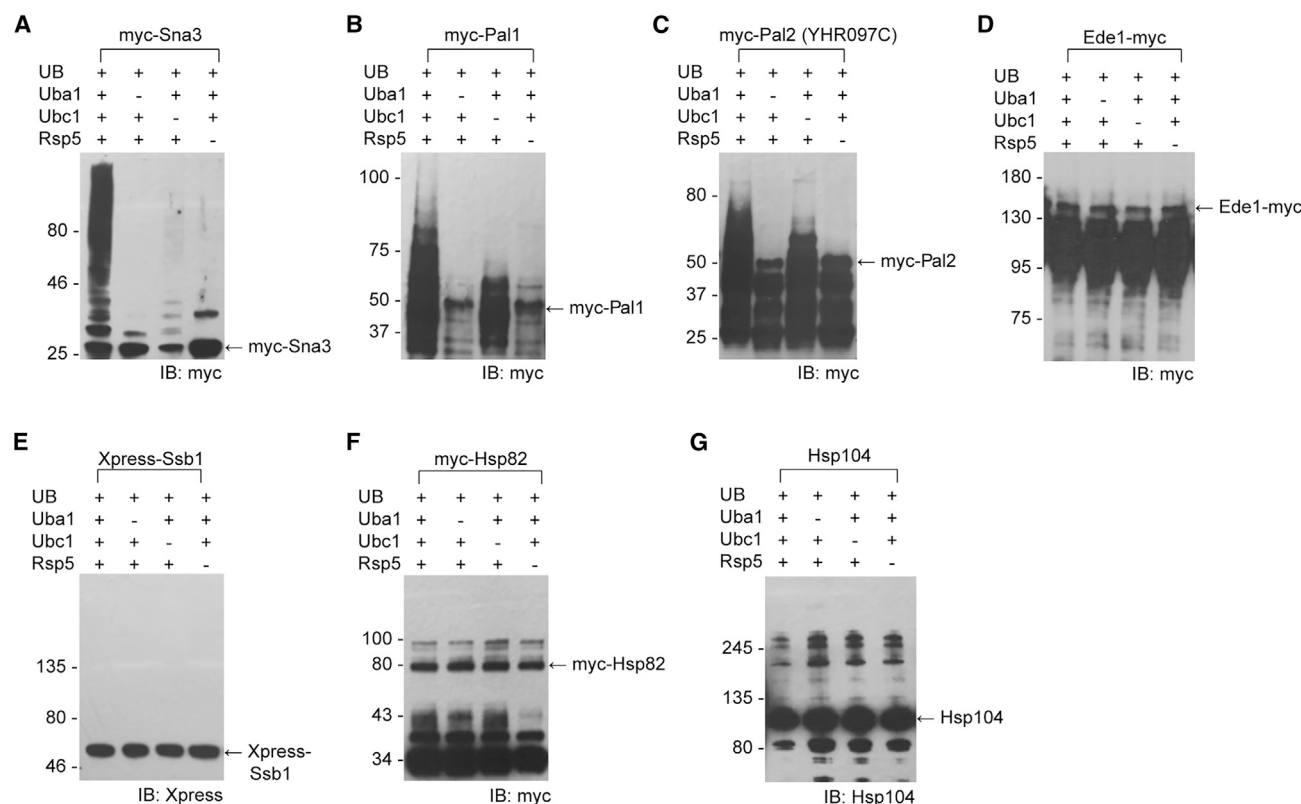
Figure 4. In vitro ubiquitination assays of the Rsp5 substrates
