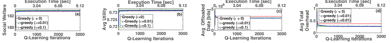
Fig. 4: Q-Learning Framework
