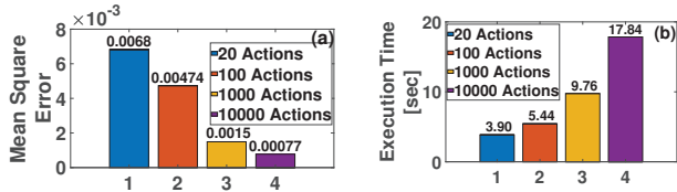
Fig. 6: Evaluation for various strategy space sizes
