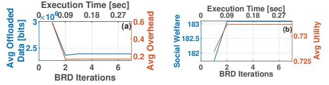
Fig. 1: Best Response Dynamics
