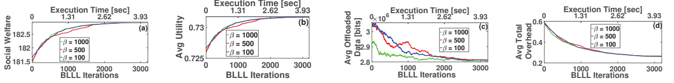
Fig. 3: Log-Linear Reinforcement Learning Framework
