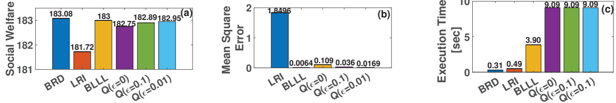
Fig. 5: Comparative Evaluation of the Reinforcement Learning Methods
