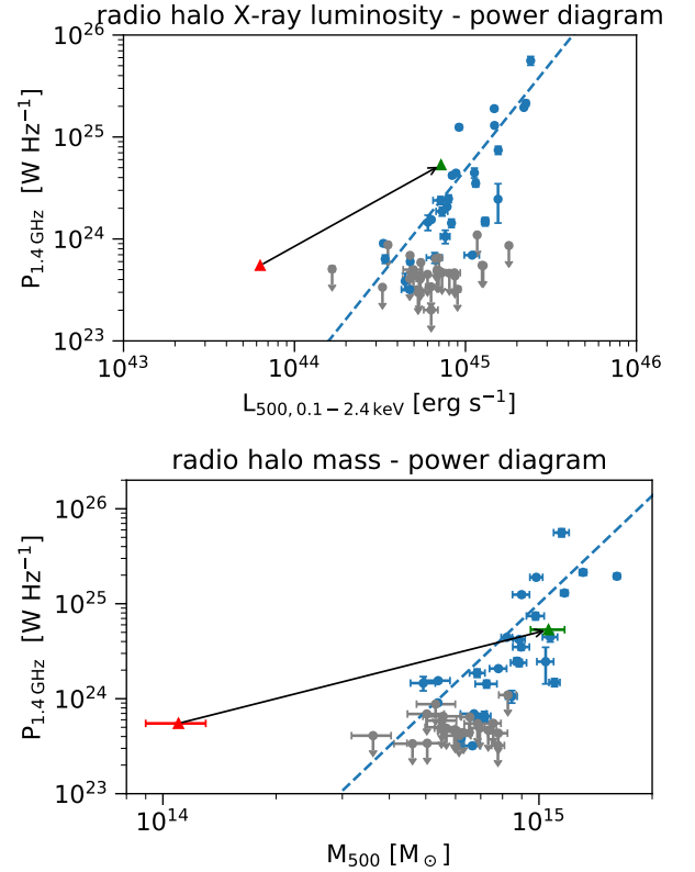
Fig. 4. L_X - P_{1.4 \text{ GHz}} (top) and M_{500} - P_{1.4 \text{ GHz}} (bottom) diagrams of radio halos. Figures are modified based on the version in van Weeren et al. (2019), where the data samples are from Cassano et al. (2013), Kale et al. (2015) and Cuciti et al. (2018). Blue points are clusters with radio halos and gray upper limits are clusters without radio halos. Blue dashed lines are the best-fit scaling relations from Cassano et al. (2013). The red triangle is CIG 0217+70 using the previous redshift, the green triangle is the corrected value. The error bars of L_X and P_{1.4 \text{ GHz}} of CIG 0217+70 are smaller than the plot symbols.
