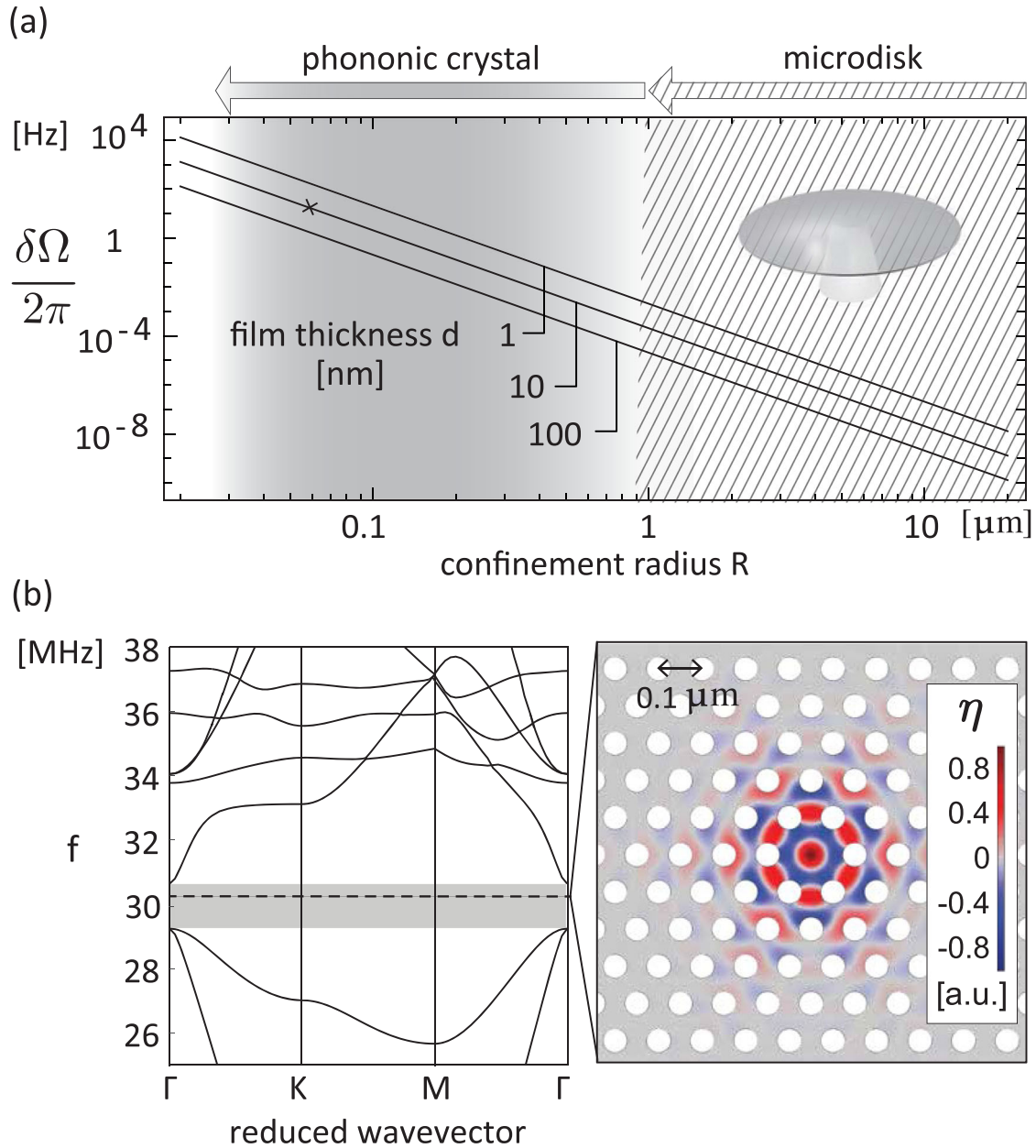
Fig. 6 Radial dependence of single-phonon shift and band structure phononic crystal. a Resonance frequency shift induced by a single phonon \delta\Omega = 3a_{\text{eff}}\chi_{\text{zpf}}^4/\hbar as a function of mode confinement radius R for various superfluid film thicknesses d for the ( \mu = 0 ; \nu = 1 ) mode. The quantized nature of the anharmonic oscillator energy spectrum is resolvable if the mechanical linewidth \Gamma < \delta\Omega . Hatched: confinement radii for microdisks 38–40,49 . Gray shaded: confinement radii achievable through phononic crystal (PnC) trapping. X-mark: mode confined in PnC cavity with lattice constant 100 nm. b PnC band structure and complete band gap (gray shaded) for a hexagonal honeycomb lattice with holes 55 nm in diameter, lattice constant 100 nm, and the van der Waals coefficient for silicon a_{\text{vdw}} = 3.5 \times 10^{-24} \text{ m}^5 \text{ s}^{-2} (ref. 60 ). A central defect (absence of hole) introduces a Bessel-like mode at 30 MHz—within the band gap—as shown by the finite-element-method simulation.
