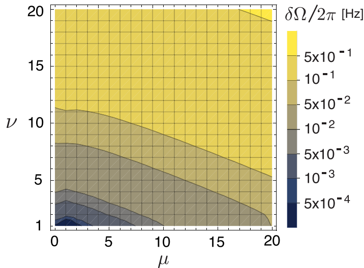
Fig. 5 Mode-number dependence of single-phonon shift. Resonance frequency shift induced by a single phonon, \delta\Omega = 3a_{\text{eff}}x_{\text{zpf}}^4/\hbar , as a function of the Bessel mode order \mu and radial node number \nu for a 5-nm-thick superfluid film confined to a 1\text{ }\mu\text{m} radius.
