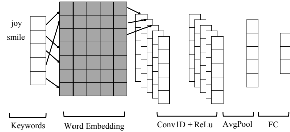
Figure 3: Architecture of text-to-emotion networks. This architecture is used by a text-to-emotion network, mapping an unordered list of keywords to a probability vector for multiple emotion categories.
