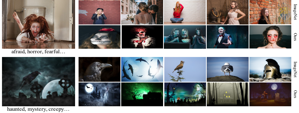
Figure 4: Two examples of images retrieved using nearest neighbour search. For each example, Left: query images and their emotion keywords. Top: returned by ImageNet features search. Bottom: returned by features trained from StockEmotion dataset.
