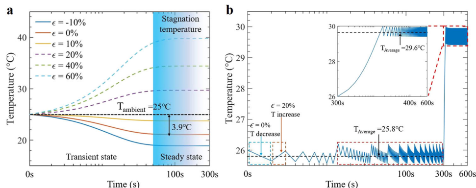
Fig. 5 Dynamic thermal regulation over time. a Stagnation temperature of the reconfigurable metamaterials as a function of strains showing the structure with tunable cooling or heating abilities under different strains. Black dashed line shows the ambient temperature is assumed to be 25^\circ\text{C} . b Transient temperature variations of the structure when subjected to dynamic mechanical strain showing the temperature can be controlled around its set temperature. The inset represents the transient temperature variations from 300s to 600s.
