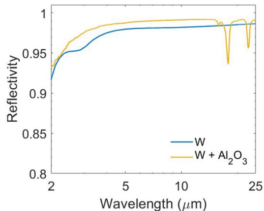
Figure 3. Spectral reflectivity of the W with and without a 100 nm thick ceramic (e.g. \text{Al}_2\text{O}_3 ) coating.
