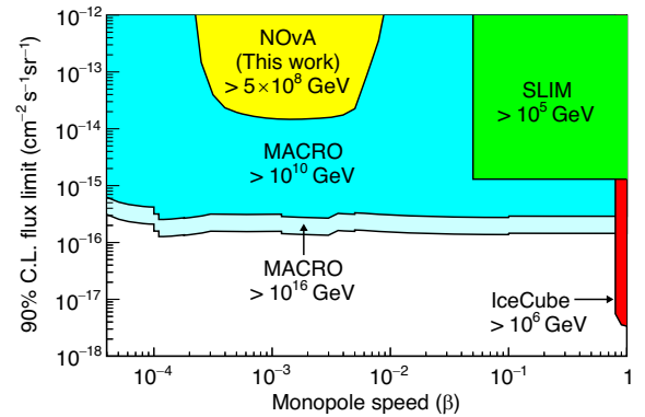
FIG. 7. Upper limits on the magnetic monopole flux. Results are shown of experiments [7,8,18] that do not assume proton decay catalysis [19] nor ultrarelativistic monopoles [20]. In each region of speed-flux space, the experiment with the best mass reach is shown. NOvA sets the only limits around \beta = 10^{-3} for monopoles lighter than 10^{10} \text{ GeV} .
