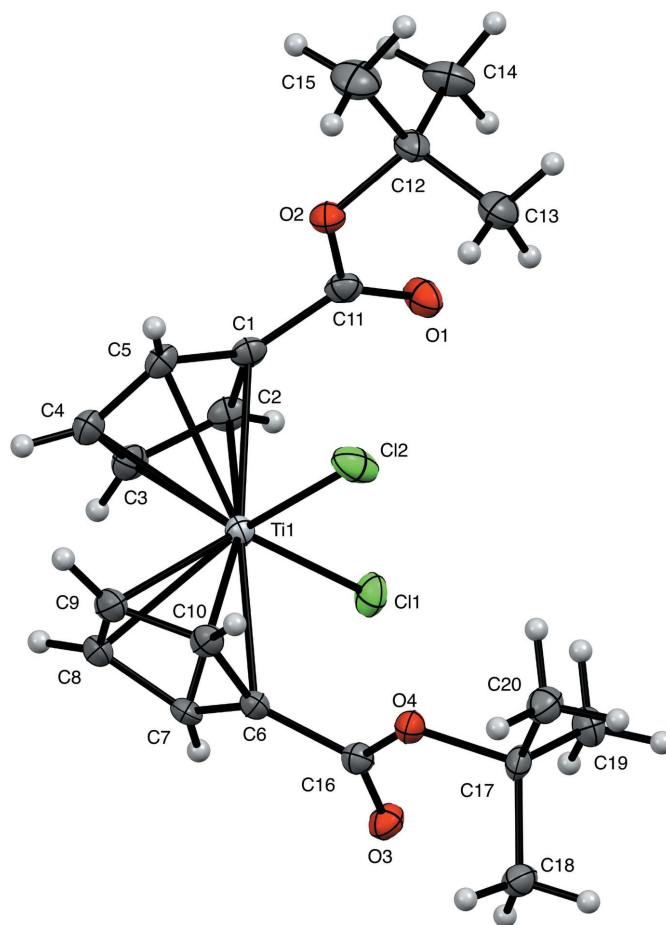
Figure 1 Structure of t\text{-BuOOC-Cp}_2\text{TiCl}_2 shown as 50% probability ellipsoids, with H atoms as small arbitrary spheres.
