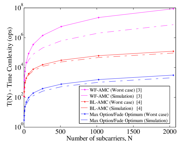
Fig. 5. Time complexity versus number of subcarriers for the adaptive models.
