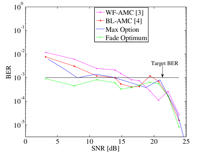
Fig. 4. Average BER versus SNR for the adaptive models.
