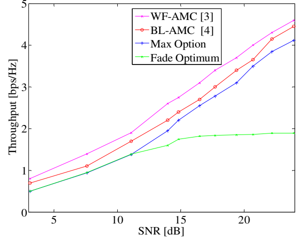
Fig.3. Average throughput versus SNR for the adaptive models.
