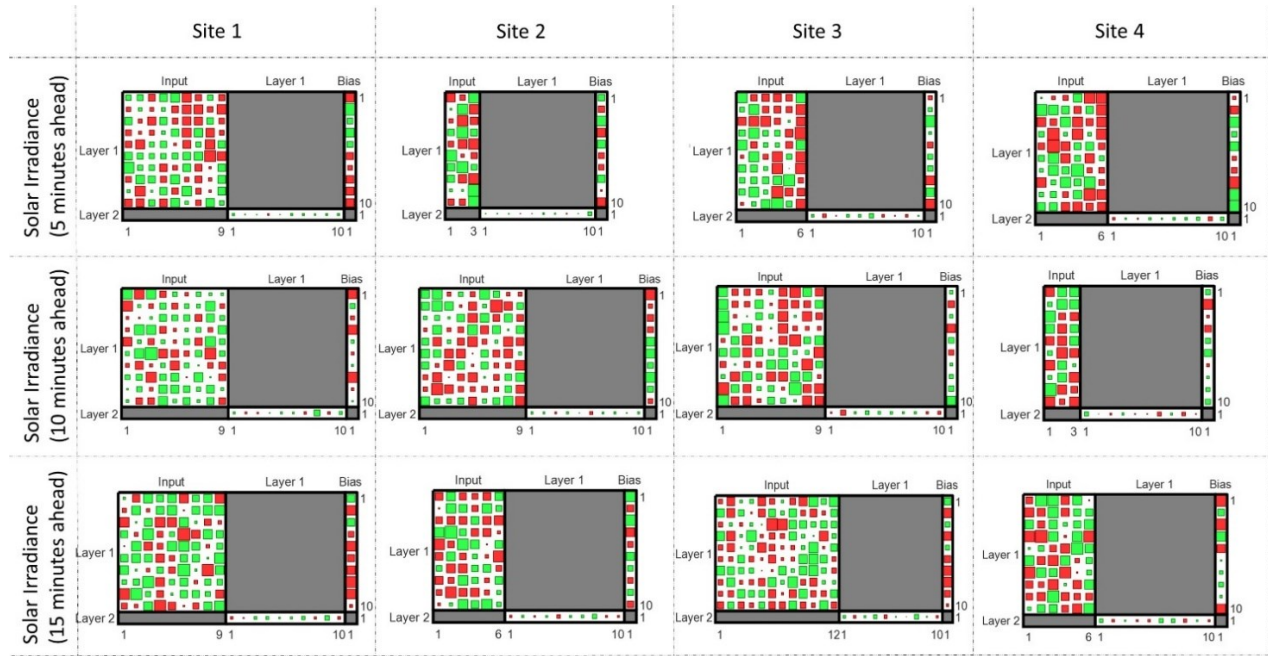
Figure 7. Hinton maps of solar irradiance predictions.
