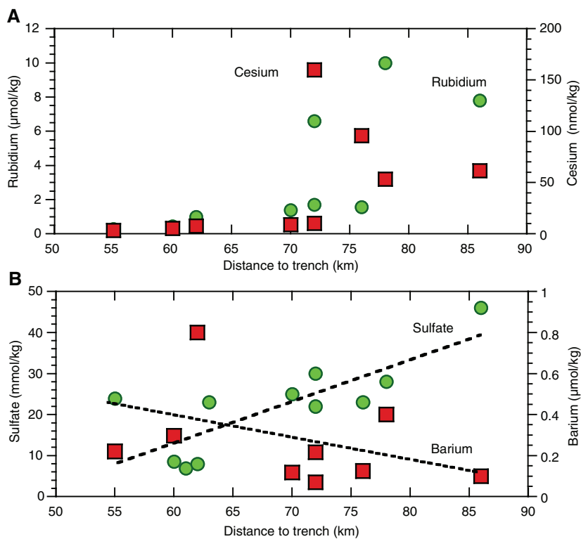
Figure F5. Concentrations of deep-sourced fluids as a function of distance to the trench. A. Trends in Rb (green circles) and Cs (red squares) are similar, showing increased concentrations with distance and by supposition depth to the subduction channel and temperature within the subduction channel. B. Trends in sulfate (green circles) and Ba (red squares) show an inverse relationship.
