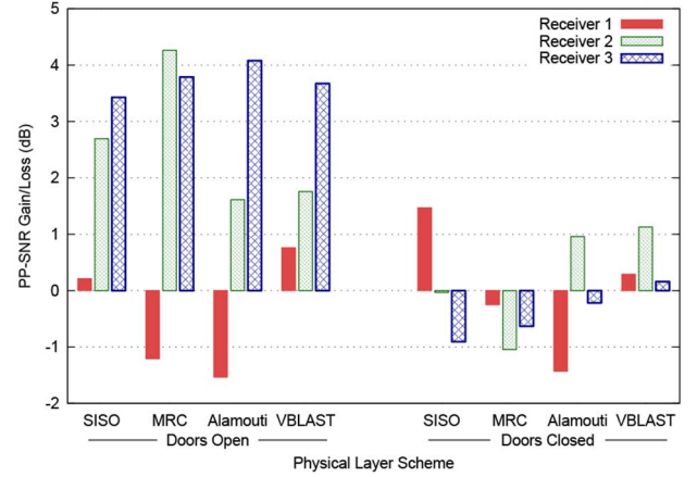
Fig. 3. PP-SNR gains (in dB) realized by switching from an omnidirectional antenna to a reconfigurable antenna at the transmitter. Gains are presented for each physical layer scheme and each receiver link with both the doors open and closed. For 10 out of 24 cases, gains of more than 1 dB are observed; For eight out of 24 cases, losses in signal quality are observed.
