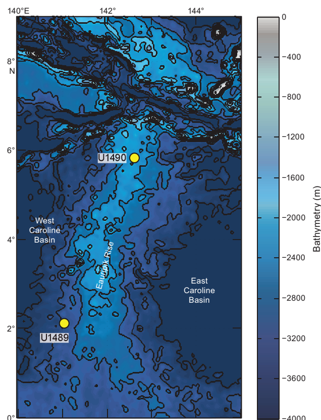
Figure F1. Bathymetric map of the equatorial Pacific Ocean indicating locations of Site U1489 (02°07.19'N, 141°01.67'E; 3400 mbsl) and Site U1490 (05°48.95'N, 142°39.27'E; 2300 mbsl) on the Eauripik Rise in the Western Pacific Warm Pool. Contour interval = 500 m. Bathymetric data from Amante and Eakins (2009); figure modified from Rosenthal et al. (2018a).
