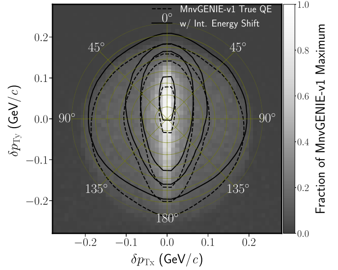
FIG. 3. \delta p_{Ty} vs \delta p_{Tx} for CCQE events in GENIE. The contours, from outside towards the center, represent 0.1, 0.2, 0.3, and 0.7 of maximum. The angles correspond to \delta \alpha_T values. The neutrino direction points out of the page. The dashed contour describes the default GENIE distribution with a MnvGENIE-v1 tune, described in Sec. V. The solid contour shows the shift in the distribution after correction is made to the interaction energy with correction 01 of Table I. There is negligible deformation in the \delta p_{Tx} direction compared to the shift in \delta p_{Ty} .
