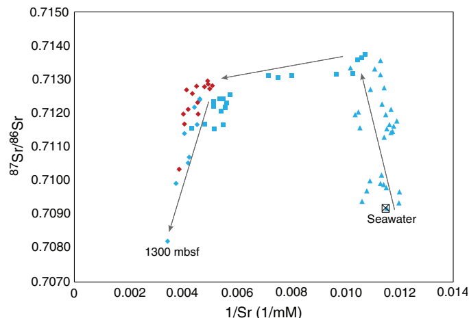
Figure F3. ^{87}\text{Sr}/^{86}\text{Sr} isotope ratios versus the inverse of Sr concentration, Sites U1480 (blue) and U1481 (red). Triangles = data from shallower than 300 mbsf, squares = data from 300 to 1100 mbsf, diamonds = data from deeper than 1100 mbsf. Only data deeper than 1100 mbsf were collected for Site U1481. Arrows point toward increasing sediment depths.
