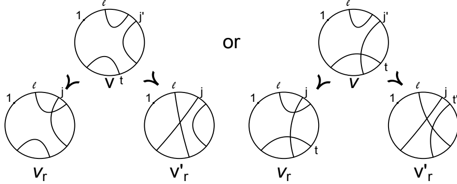
FIGURE 10. v_r \prec v and v'_r \prec v
