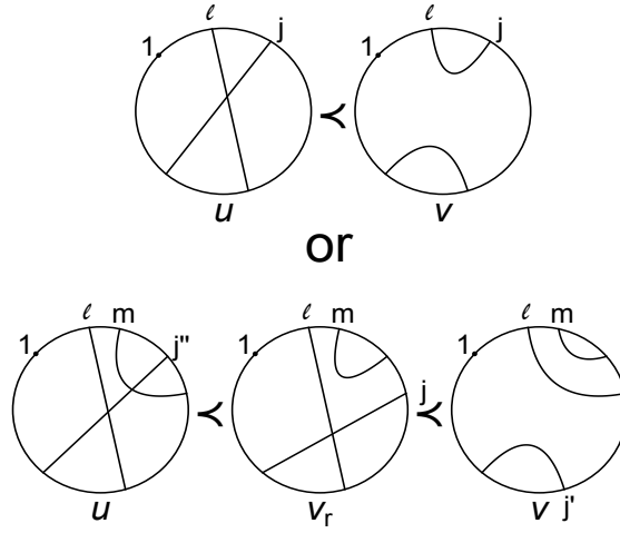
FIGURE 9. \lambda(v_r, v) = (j, l)
