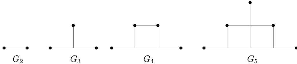
FIGURE 16. The well connected graphs G_2 , G_3 , G_4 and G_5
