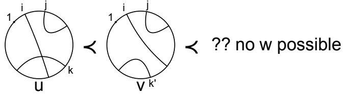
FIGURE 14. Case d: cannot arise due to contradiction
