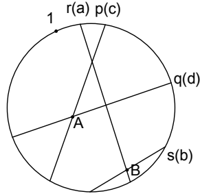
FIGURE 6. x \prec y and y' \prec z uncrossings at A ; x \prec y' and y \prec z uncrossings at B
