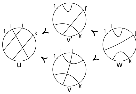
FIGURE 11. Case a: u \prec v \prec w topological ascent
