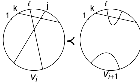
FIGURE 8. \lambda(v_i, v_{i+1}) = (j, l)
