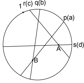
FIGURE 5. x \prec y' and y \prec z uncrossings at A ; x \prec y and y' \prec z uncrossings at B
