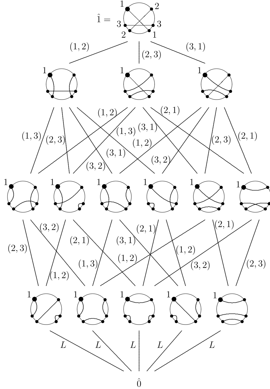
FIGURE 7. Dual EC labeling for P_3
