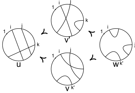
FIGURE 13. Case c: u \prec v \prec w topological descent
