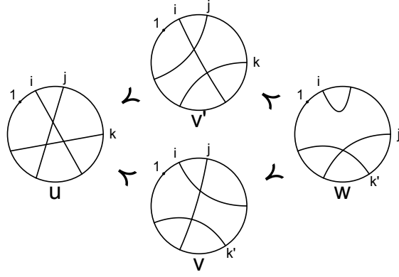
FIGURE 12. Case b: u \prec v \prec w topological descent
