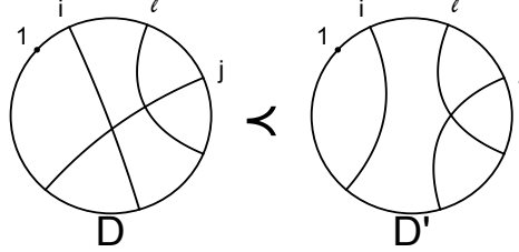
FIGURE 15. \lambda(D, D') = (i, j)
