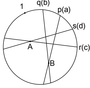
FIGURE 4. u \prec z and x \prec y' uncrossings at A ; x \prec y and y' \prec z uncrossings at B
