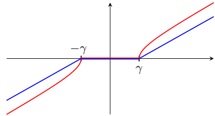
Fig. 4. The threshold (16) of [15] (red) and the soft thresholder (blue) used in Section III-B.
