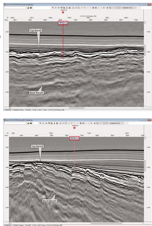
Figure AF17. Track map and seismic profiles, primary Proposed Site VMVM-61A. SP = shotpoint. SSDB = Site Survey Data Bank.
