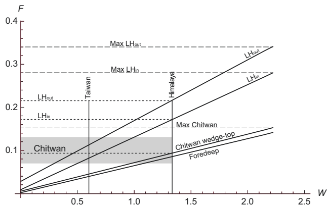
Figure 10. Plot of dimensionless fault strength ( F ) versus wedge strength ( W ) (Suppe, 2007). Sloping lines are functions from Table 1. Lines terminate at maximum W values corresponding to \tan \phi = 0.85 (Byerlee's law). Horizontal dashed lines indicate corresponding maximum values of F for different sectors of the Himalayan wedge labeled as follows: Max LH out —Lesser Himalayan wedge outside of the erosional bight; Max LH in —Lesser Himalayan wedge inside the erosional bight; Max Chitwan—the sector of the wedge in the Chitwan wedge-top basin area. Gray area represents range of fault strength values determined by Cattin and Avouac (2000), Avouac (2007), and Dal Zilio et al. (2019) for the Himalayan basal décollement. Vertical line labeled Taiwan is wedge strength of the Taiwan orogenic wedge from Suppe (2007). Vertical line labeled Himalaya is value of W calculated for \phi = 30^\circ , and dotted horizontal lines indicate corresponding values of F as discussed in text.
