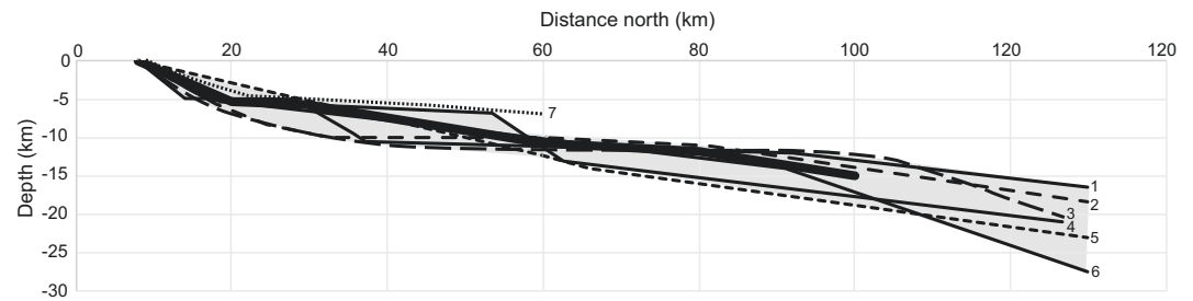
Figure 8. Cross-section profile across the central Nepal thrust belt showing interpreted locations of the basal Himalayan décollement in publications listed. Numbered profiles correspond to the following sources: 1, DeCelles et al. (2020); 2, Nábělek et al. (2009); 3, Duputel et al. (2016); 4, Khanal and Robinson (2013); 5, Schulte-Pelkum et al. (2005); 6, Elliott et al. (2016); 7, Figure 3 of this paper. Gray area indicates complete range of interpretations and bold line is our mean approximation. See text for discussion.
