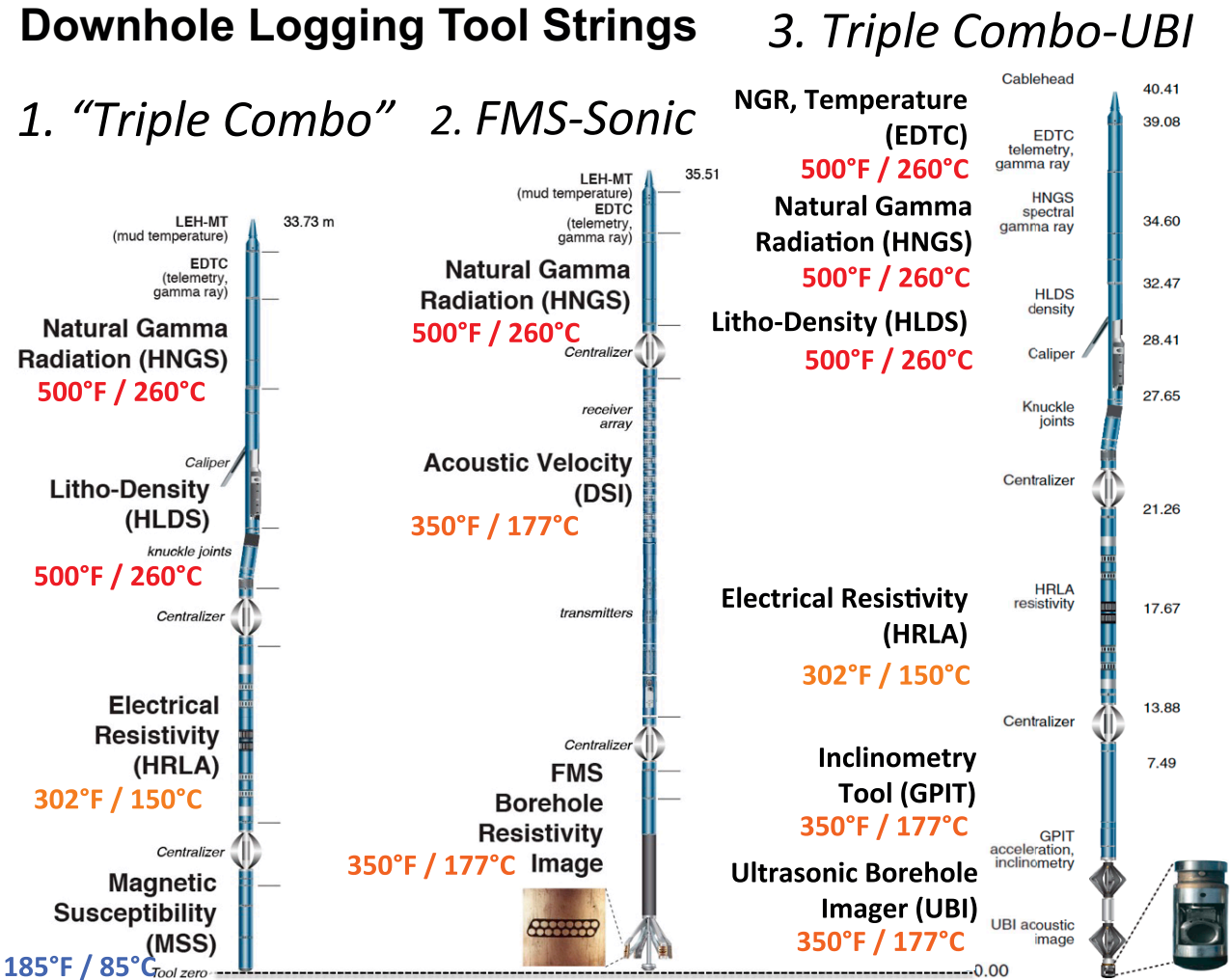
Figure F5. Standard wireline logging tool suites available on board JOIDES Resolution : triple combo, FMS-sonic, and triple combo-Ultrasonic Borehole Imager (UBI) downhole logging tool strings (see http://iodp.tamu.edu/tools/logging ), including published tool temperature ratings (in both °F and °C). The triple combo and FMS-sonic tool strings are intended for use during Expedition 385 wireline logging (if formation temperature permits). Temperatures refer to the maximum temperature level of the corresponding tool. LEH-MT = logging equipment head-mud temperature, EDTC = Enhanced Digital Telemetry Cartridge, NGR = natural gamma radiation, HNGS = Hostile Environment Natural Gamma Ray Sonde, HLDS = Hostile Environment Litho-Density Sonde, HRLA = High-Resolution Laterolog Array Tool, MSS = Magnetic Susceptibility Sonde, DSI = Dipole Sonic Imager, FMS = Formation MicroScanner (borehole microresistivity imager), GPIT = General Purpose Inclinerometry Tool.
